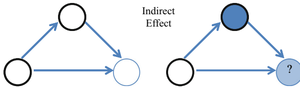
Fig. 4 White circles default values. Filled circles non-default values. Question mark value unknown. Black halos interventions. The indirect effect is derived by subtracting the expected value of the outcome on the left from that on the right
