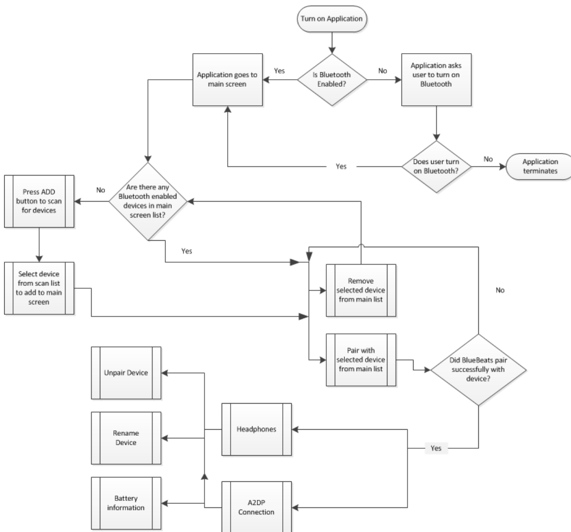
Figure 1: Software Flowchart
