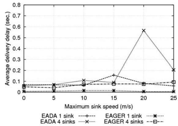
Fig. 10 Average delivery delay vs. maximum sink speed
