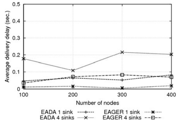
Fig. 11 Average delivery delay vs. number of nodes
