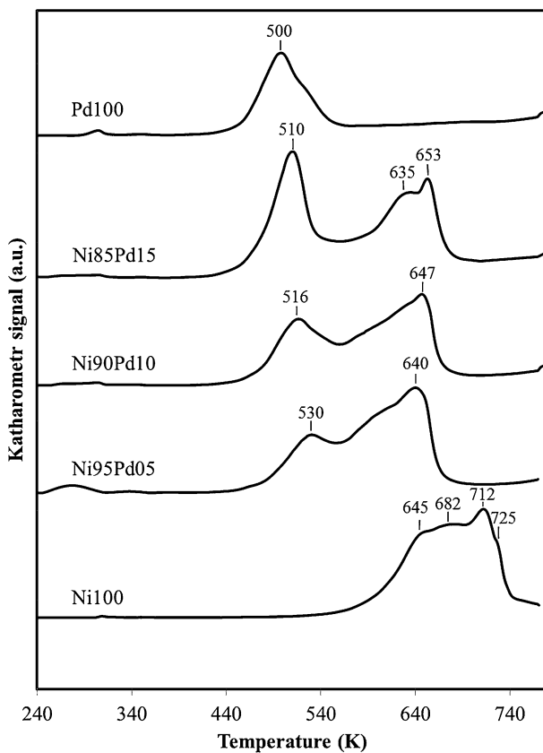
Fig. 1 Temperature programmed reduction (TPR) profiles of Norit CNR115-supported Pd–Ni catalysts
