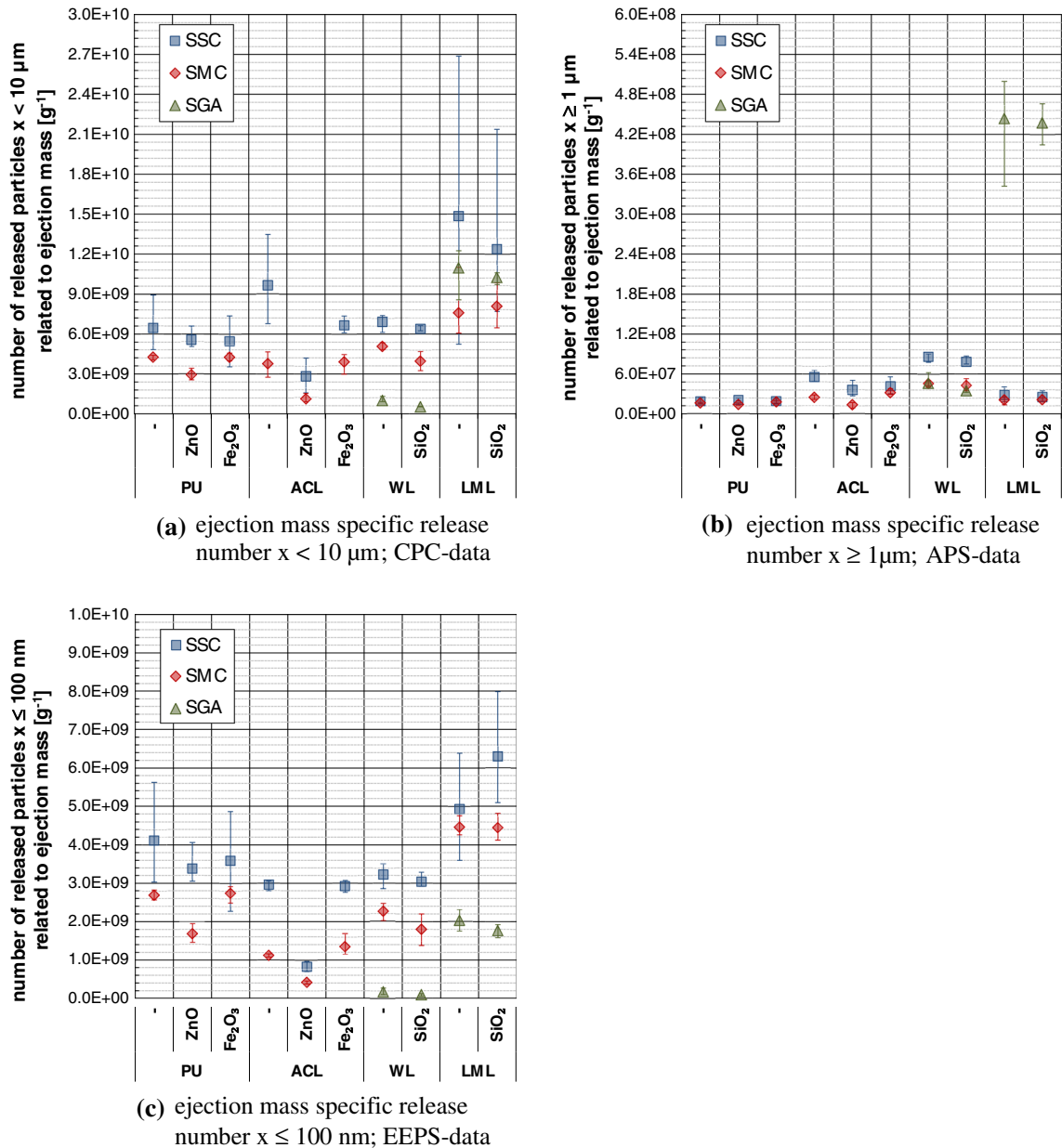
Fig. 9 Ejection mass specific fractional numbers of released particles; error bars = data spreading of 5 (SGA) and 6–12 (SSC, SMC) repeated measurements
