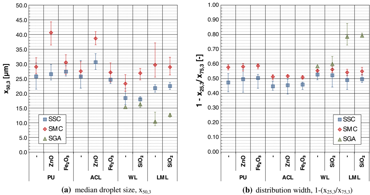
Fig. 6 Characteristic parameters of the volume-weighted droplet size distribution ( PSD_3 ) at a distance of 10 mm from the nozzle exit, determined by laser diffraction analyzes; error bars = spreading of 15 repeated measurements
