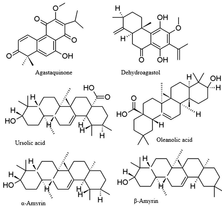
Fig. 5 Structures of diterpenoids and pentacyclic triterpenes from Agastache
