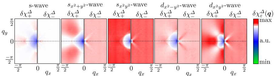
Fig. 3 Change in the static Cooper pairs susceptibility \delta\chi_\varepsilon^\Delta(\mathbf{q}) (for data presented in Fig. 2 (Color figure online))
