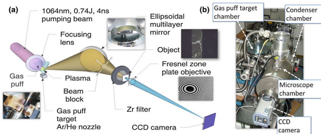
Fig. 1 a Scheme (not to scale) and b photograph of the EUV microscope using a laser-plasma EUV source based on gas-puff target
