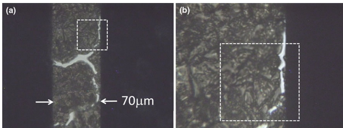
Fig. 2 Optical images of thin Si membrane with NaCl crystals deposited on top with a 40\times ( \text{NA} = 0.65 ), b 100\times ( \text{NA} \sim 1 ) objectives. Dashed boxes indicate the size of object region imaged with the EUV microscope
