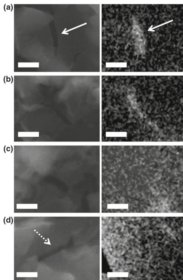
Fig. 4 Comparison between small sections of SEM images ( left column ) and EUV images ( right column ) showing different areas of the sample. a, b Some cracks, as small as 100 nm, in the sample are deep all the way to the membrane and can be seen in both SEM and EUV images (marked with white arrows and c, d some of the features (marked with dotted arrow ) are visible in the SEM images but are not present in the corresponding EUV image. Scale bar is 2 \mu\text{m}
