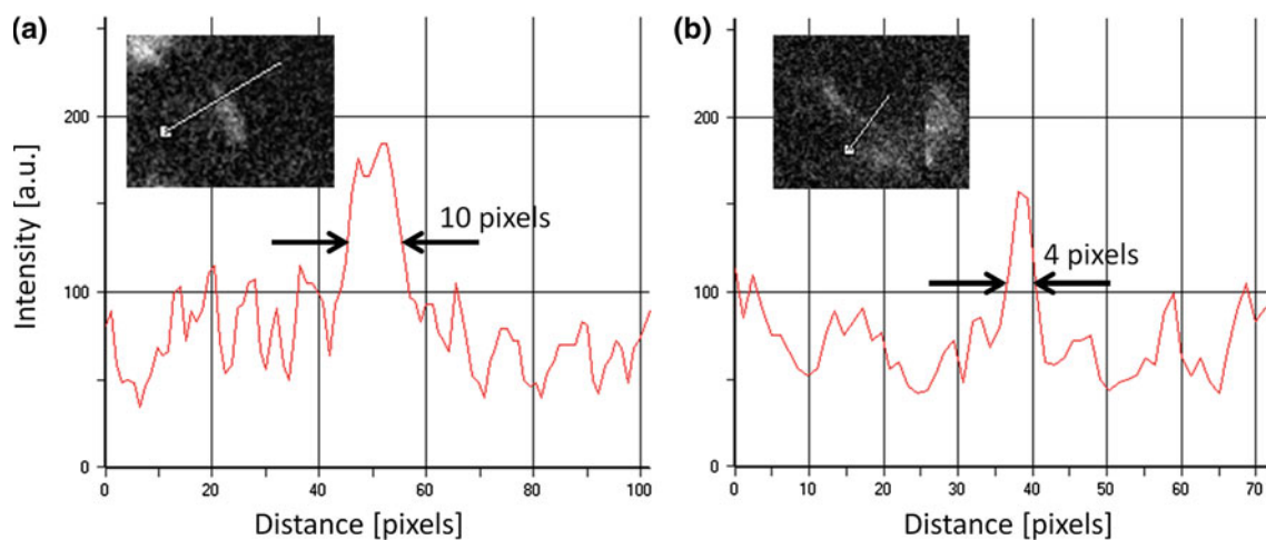
Fig. 5 Intensity profiles of smallest features in the EUV images (a) showing visible features as small as 4 pixel wide (b)
