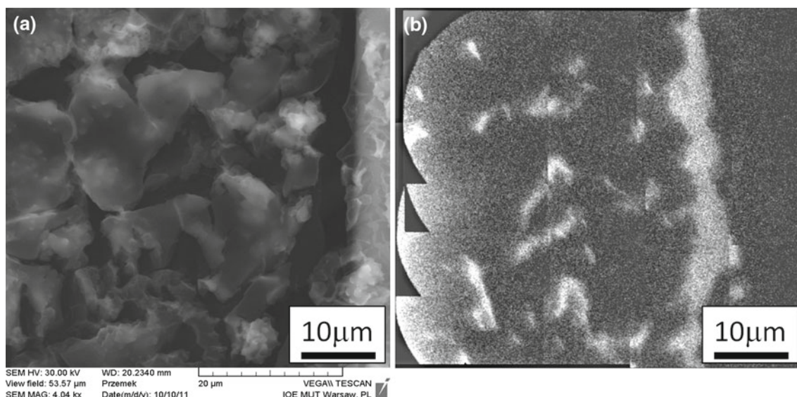
Fig. 3 SEM image of the sample, \sim 50 \times 50\text{ }\mu\text{m}^2 with re-crystallized NaCl (a) and corresponding EUV image (b) showing the same region of the sample. EUV image was obtained by stitching and partially overlapping of 4 \times 4 smaller EUV sub-images
