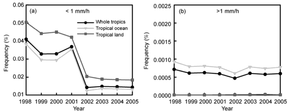
Figure 5 Same as in Figure 3 but for other-type precipitation.
