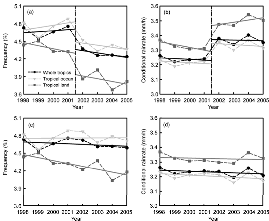
Figure 7 Interannual variations of precipitation frequency ((a), (c)) and conditional rainrate ((b), (d)) before ((a), (b)) and after ((c), (d)) correction.
