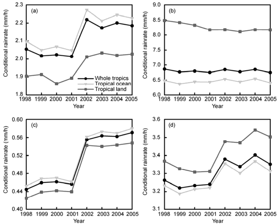
Figure 2 Same as in Figure 1 but for conditional rainrate.
