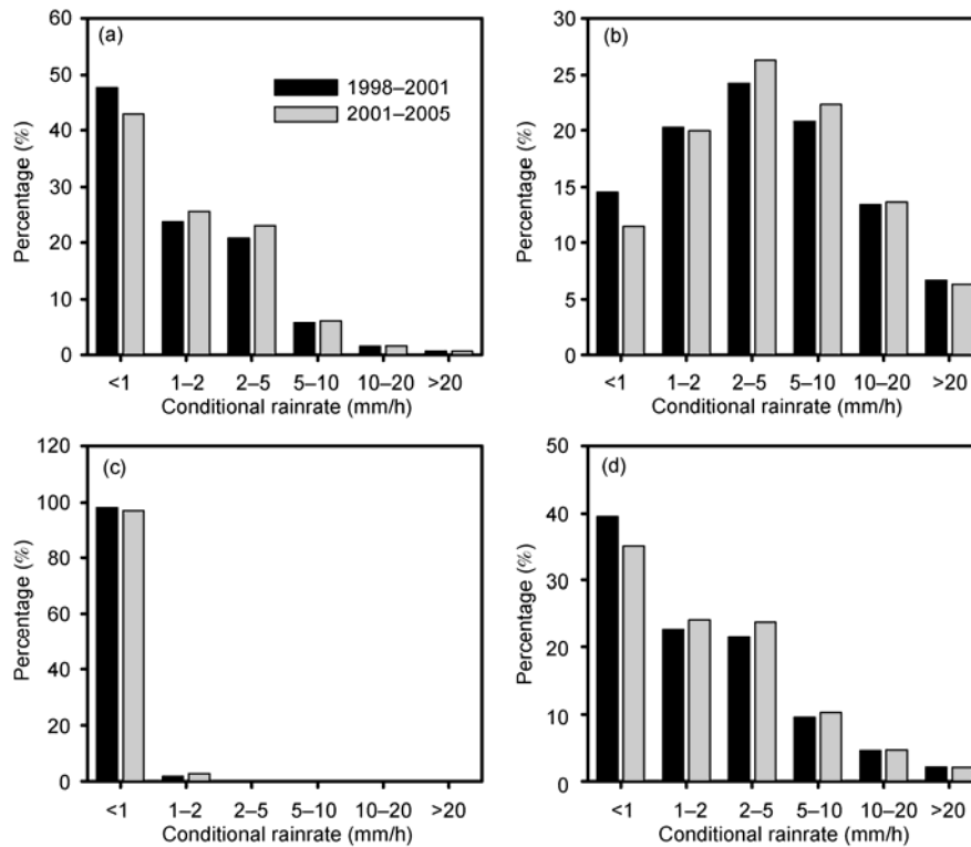
Figure 6 Precipitation intensity spectrums of pre- and post-boost periods for (a) stratiform precipitation, (b) convective precipitation, (c) other-type precipitation, and (d) all-type precipitation.
