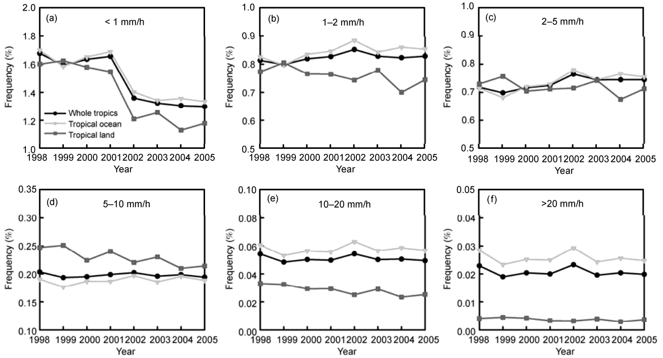
Figure 3 Interannual variations of stratiform precipitation frequency in different rainrate segments.
