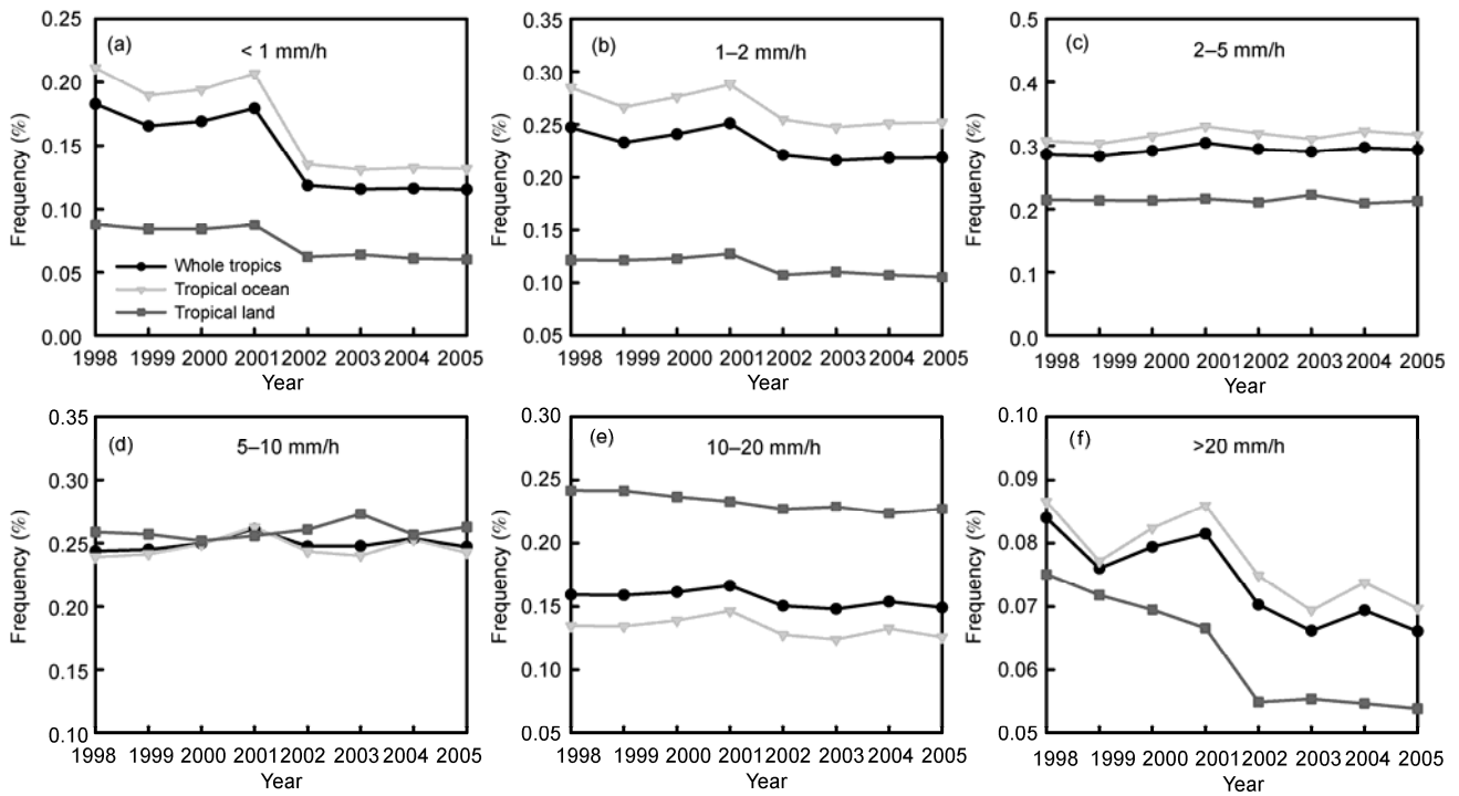
Figure 4 Same as in Figure 3 but for convective precipitation.
