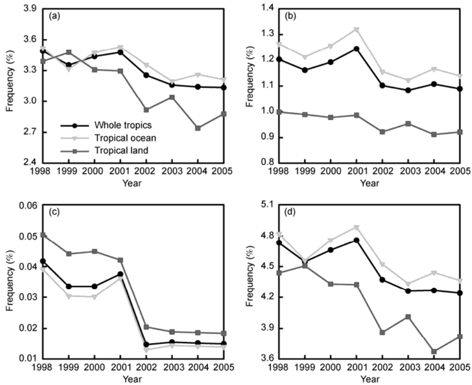
Figure 1 Interannual variations of precipitation frequency for stratiform precipitation (a), convective precipitation (b), other-type precipitation (c), and all-type precipitation (d).
