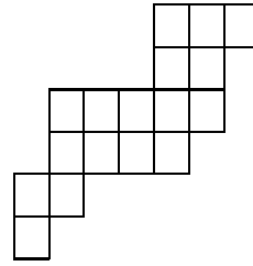
Parallelogram Polyomino: No lower or upper descents
