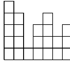
Wall Polyomino: No lower ascents and no lower descents
