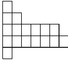
Stack Polyomino: No upper ascents and no lower descents
