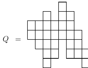
Diagram 3: A Column-Convex Polyomino
