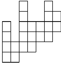
Directed Column-Convex Polyomino (DCCP): No lower descents
