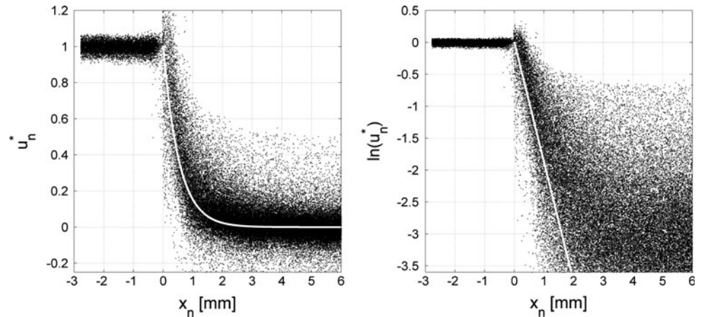
Fig. 12 Scatter plot of individual particles velocity across the shock. Linear ( left ) and logarithmic ( right ) diagrams
