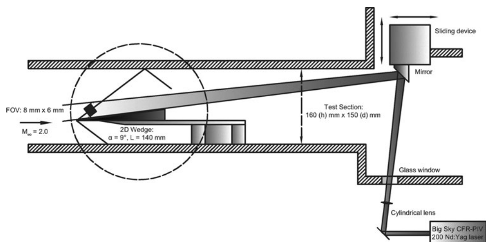
Fig. 7 Test section, illumination and imaged region
