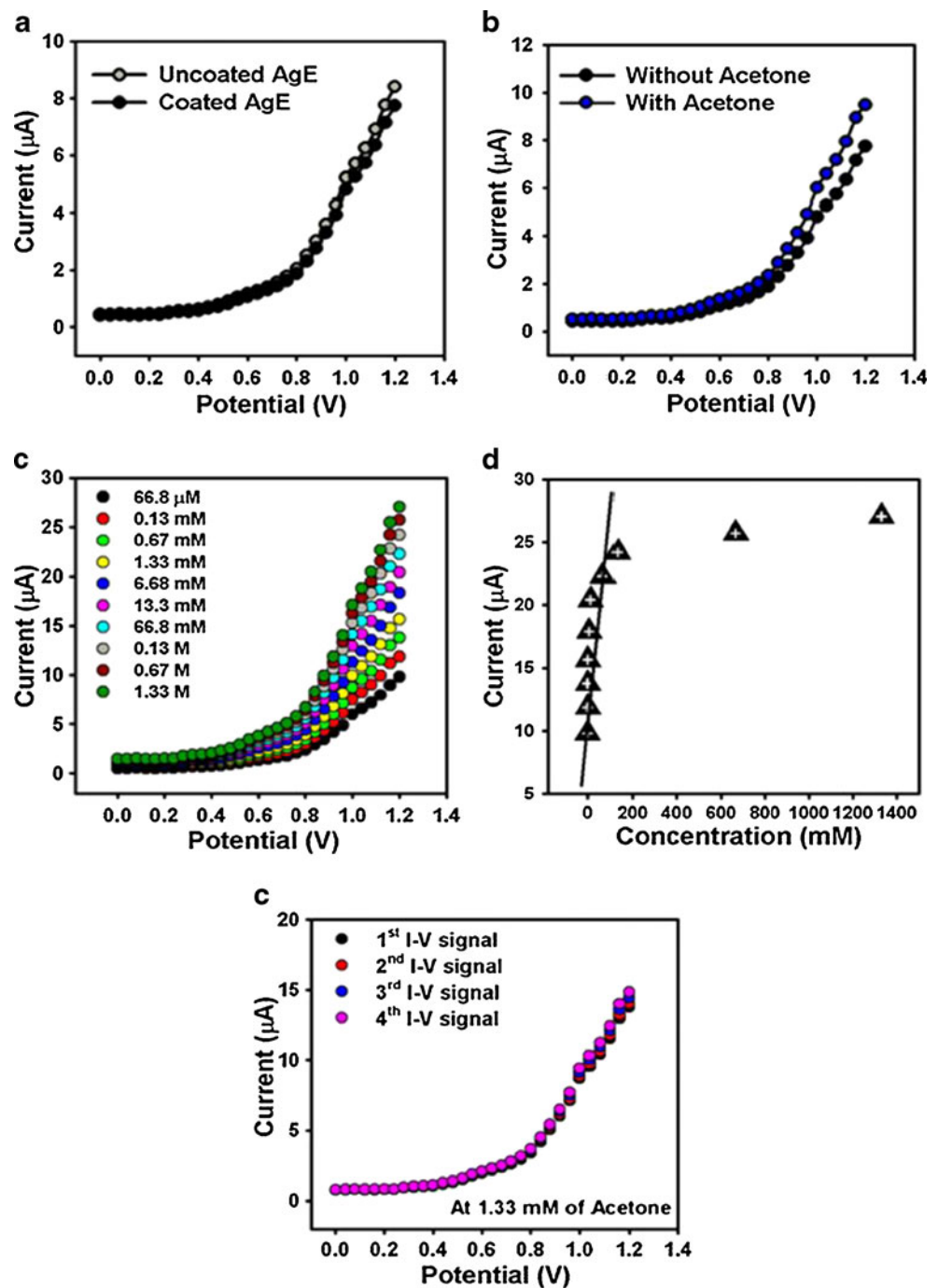
Fig. 4 I-V responses of a uncoated and coated AgE; b without and with acetone (66.8 \mu\text{M} ) in 10.0 mL phosphate buffer solution; c concentration variations (66.8 \mu\text{M} to 1.33 M) of acetone; d calibration plot (at +0.7 V), and e repeatability signals of ZnO-doped \text{Co}_3\text{O}_4 NRs fabricated on AgE surfaces. Potential was between 0.0 and +1.2 V
