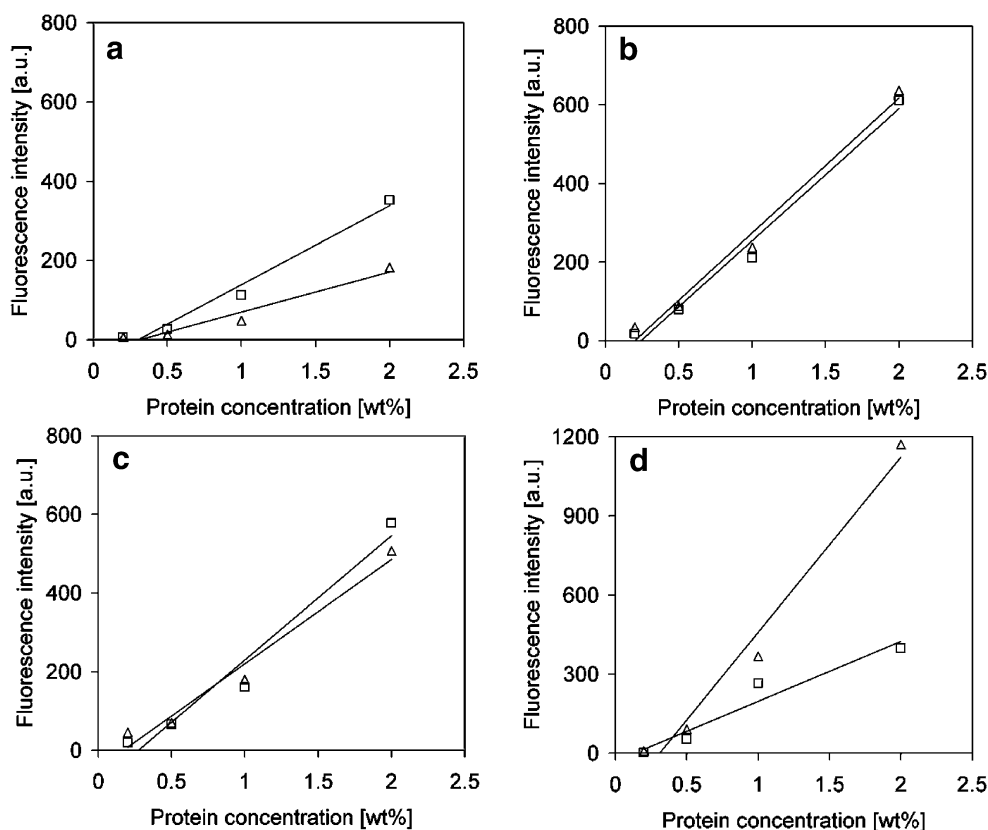
Fig. 3 The protein concentration versus the conversion into fibrils of \beta -lg solutions (pH 2) heated at 343 K (a), 358 K (b), 363 K (c), and 383 K (d). The solutions were stirred at 290 rpm (open squares) or stirred at 1,200 rpm (open triangles) during heating
