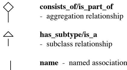
Figure 6: UML Relationships
