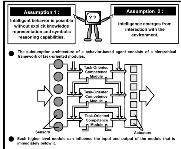
Figure 4: Subsumption architecture
