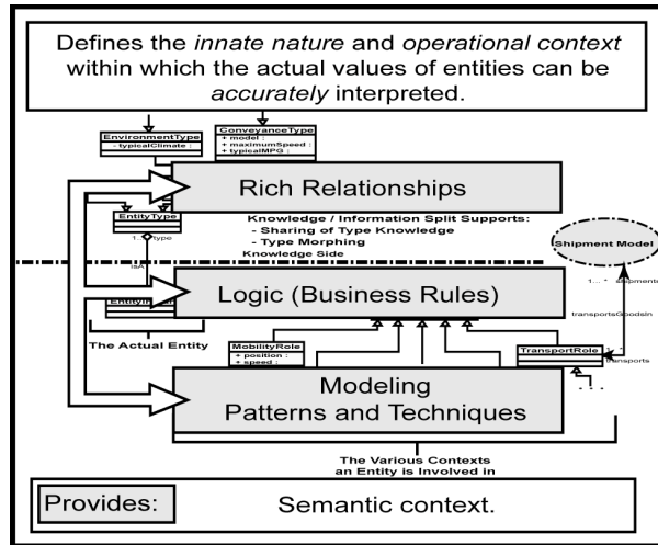
Figure 2: Ontology representation
