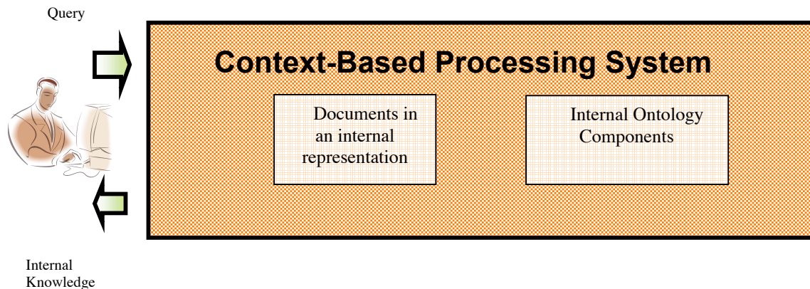
Figure 4: Query Module.
