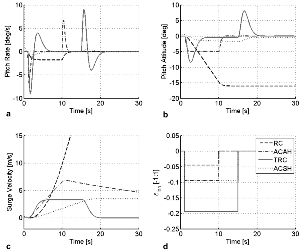
Fig. 1 Response types used for PAV flight dynamics model. The vehicle model was also equipped with pilot-selectable heading and height hold autopilot functions
