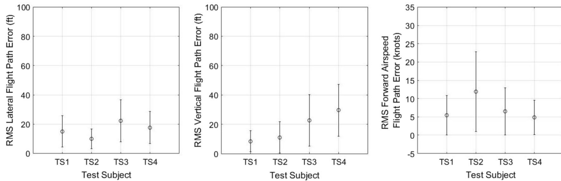
Fig. 8 Deviation from desired flight path during the commute scenario flight test
