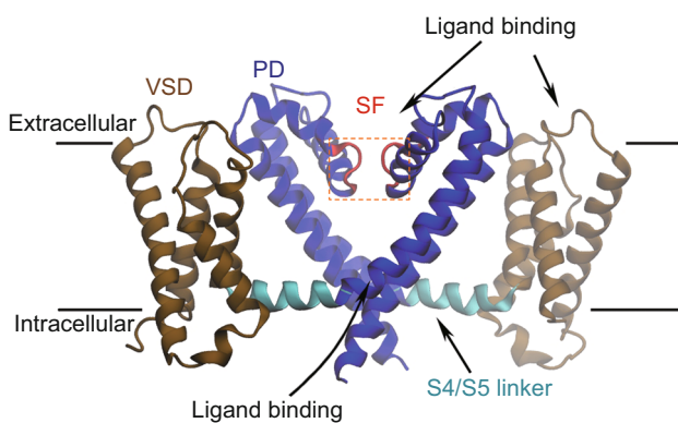
Figure 1. The structural organization of VGCCs. Only the opposing two TDs are shown to facilitate visual recognition. The PD (purple) and VSDs (brown) are connected by a half helix (cyan) between TMs S4 and S5. The SF region within the PD is colored in red. Ligands can bind at both PD and VSDs, as shown by the black arrows.
