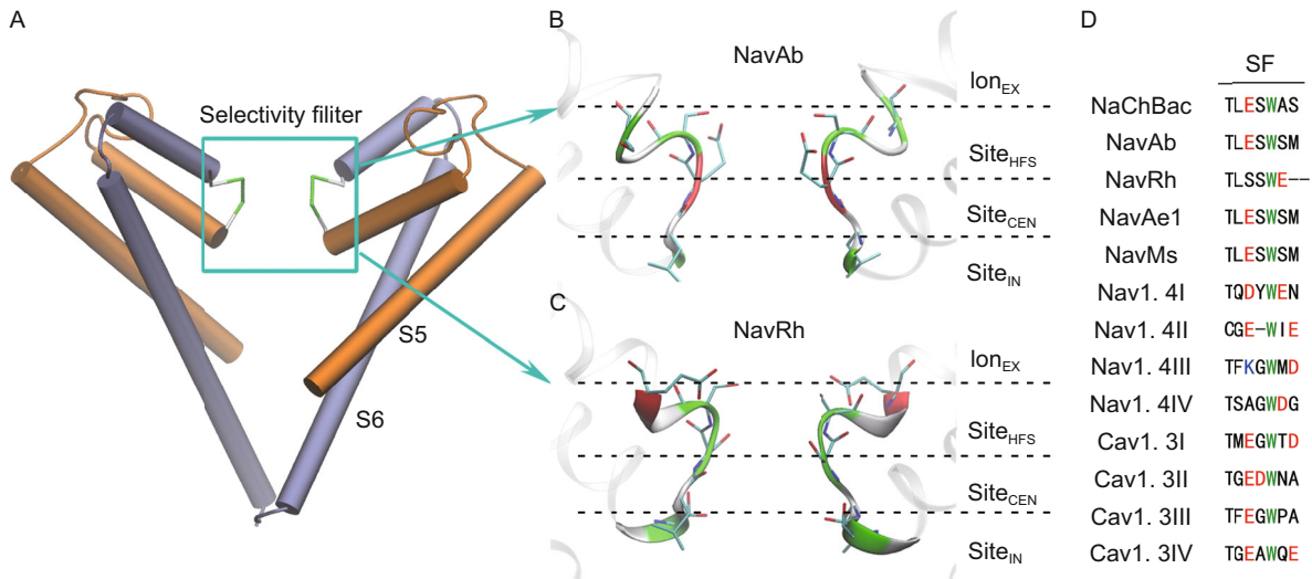
Figure 2. The ion binding sites identified in the SF of \text{Na}_v channels. (A) The SF region is labeled by a cyan frame. (B) The schematic ion binding sites in \text{Na}_v\text{Ab} . (C) The schematic ion binding sites in \text{Na}_v\text{Rh} . (D) Aligned amino acid sequences for the SF region in various prokaryotic \text{Na}_v channels as well as eukaryotic \text{Na}_v and \text{Ca}_v channels. The four structural units in the eukaryotic channels are labeled as I, II, III and IV, respectively.
