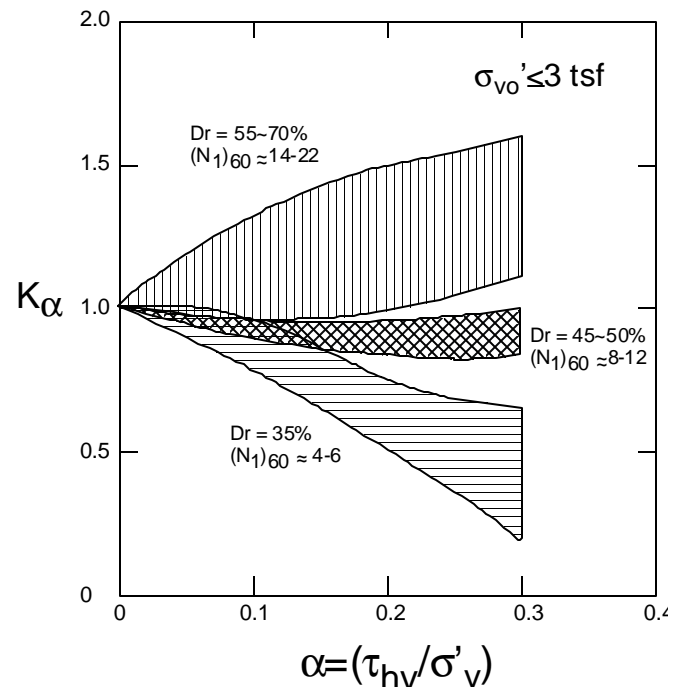
Fig. 39: Recommended Values of K_{\hat{a}} as a Function of SPT N-Values for Effective Vertical Stresses of Less Than 3 atmospheres (After Harder and Boulanger, 1997)
