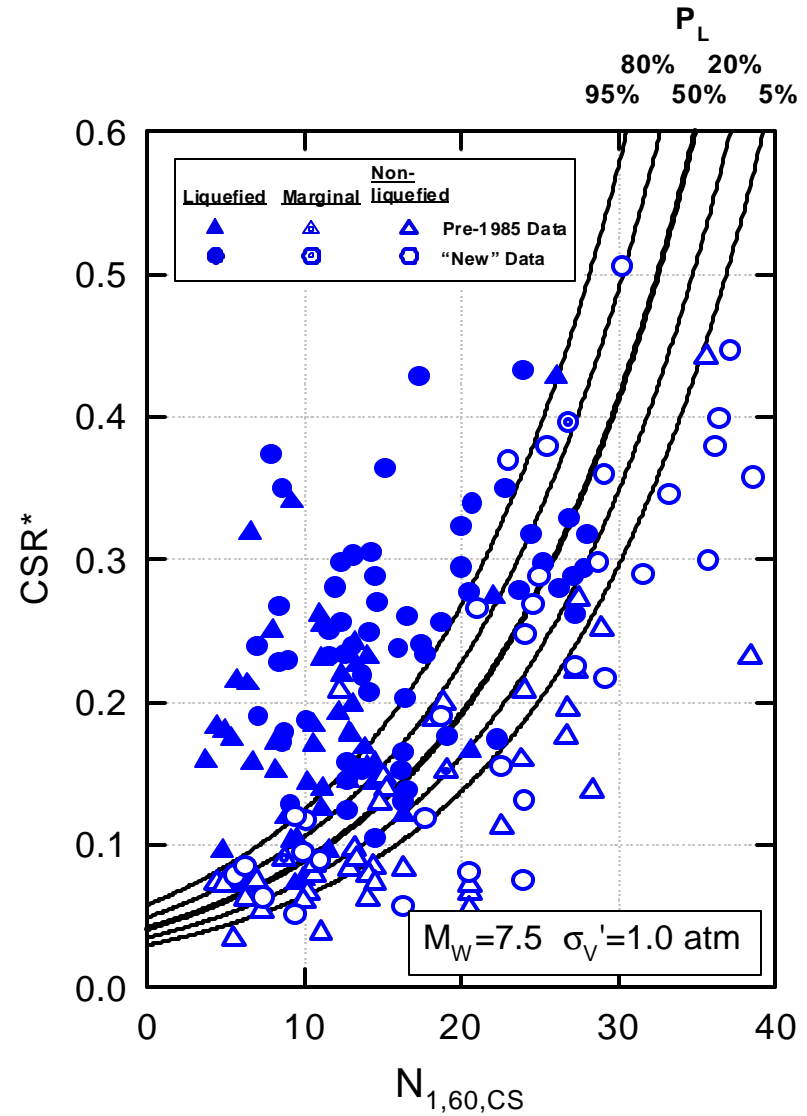
Fig. 25: Contours of 5%, 20%, 50%, 80% and 95% Probability of Liquefaction for \hat{q}' = 1 \text{ atm} and Duration Associated with M_w = 7.5 As a Function of Fines Corrected SPT Penetration Resistance (Seed et al., 2001)
