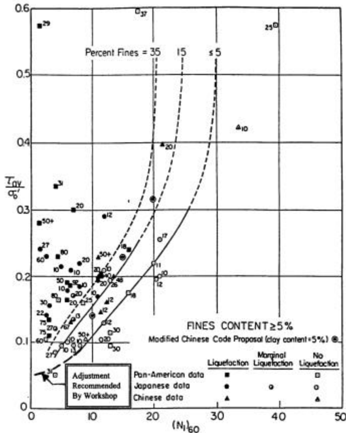
Fig. 5: Correlation Between Equivalent Uniform Cyclic Stress Ratio and SPT N_{1,60} -Value for Events of Magnitude M_w 7.5 for Varying Fines Contents, With Adjustments at Low Cyclic Stress Ratio as Recommended by NCEER Working Group (Modified from Seed, et al., 1984)
