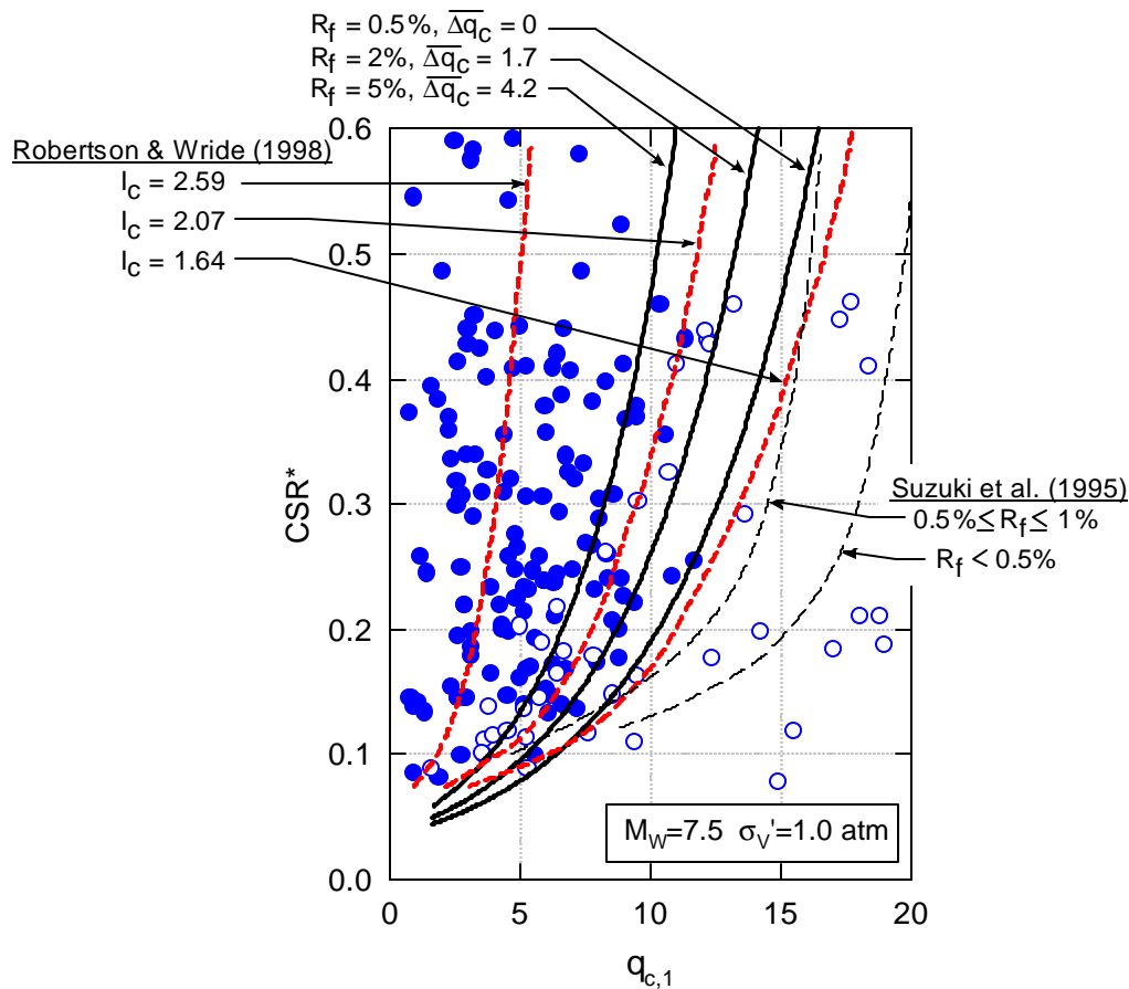
Fig. 31: Comparison Between the Recommended New CPT-Based Correlation and Previous Relationships Proposed by Suzuki et al. (1995) and Robertson and Wride (1998) [ M_w=7.5 , \sigma_v'=1 atm.]
