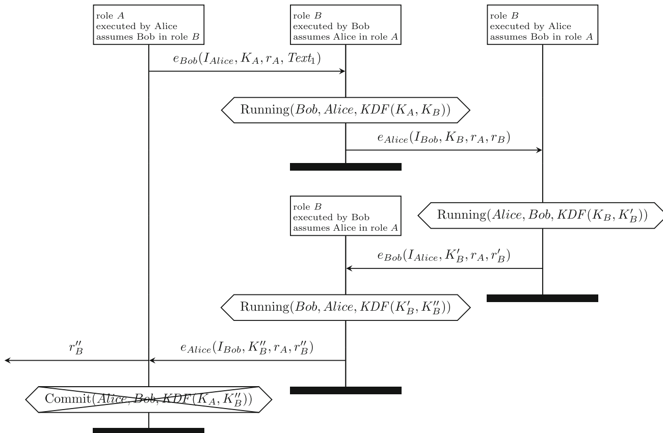
Fig. 8 3-KT-6 combined key variant with Text_1 optional field key confirmation attack
