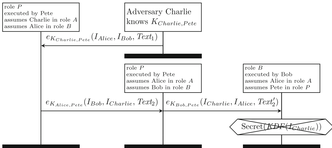
Fig. 6 Protocol 2-11 key authentication attack
