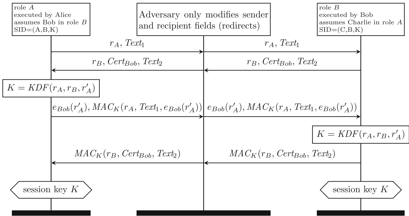
Fig. 9 Unknown key share attack on protocol 3-KA-11. Alice shares a key K with Bob as she expects, but Bob mistakenly assumes he shares K with Charlie
