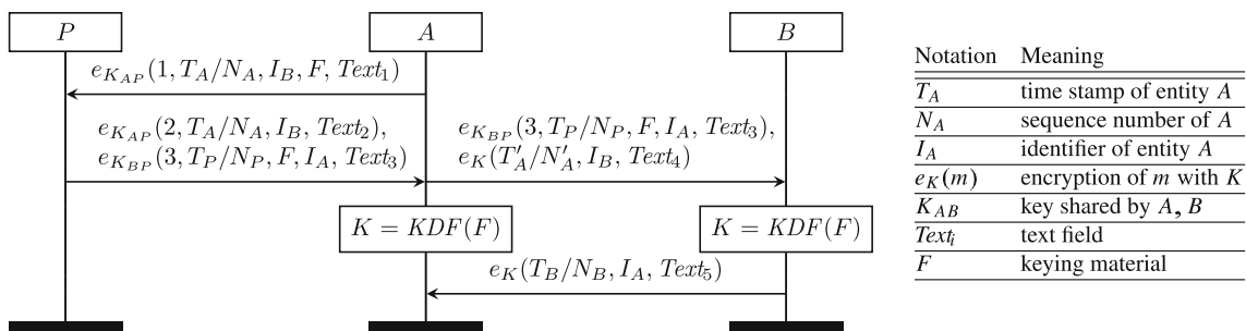
Fig. 1 Protocol 2-12 with optional parts
