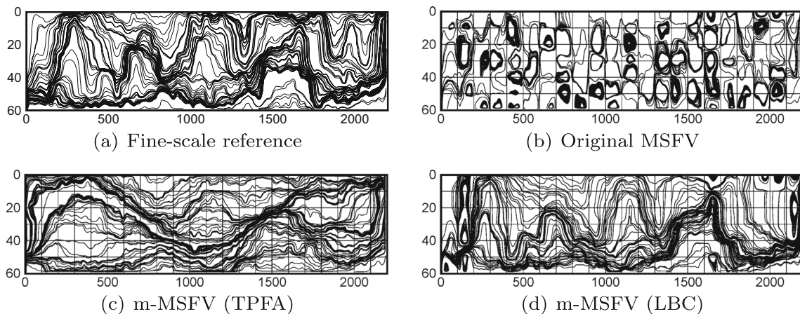
Fig. 18 Streamline plots based on velocity fields reconstructed by fine-scale reference, original and monotone MSFV pressure solutions
