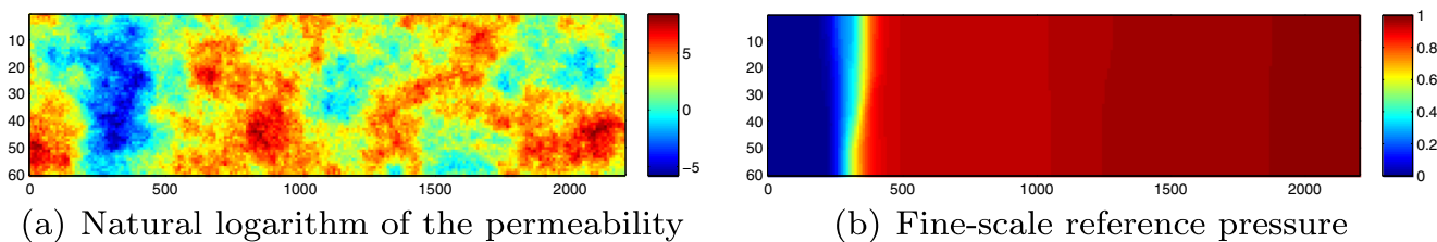
Fig. 16 Permeability and fine-scale pressure solution for the SPE 10 top layer with stretched grids
