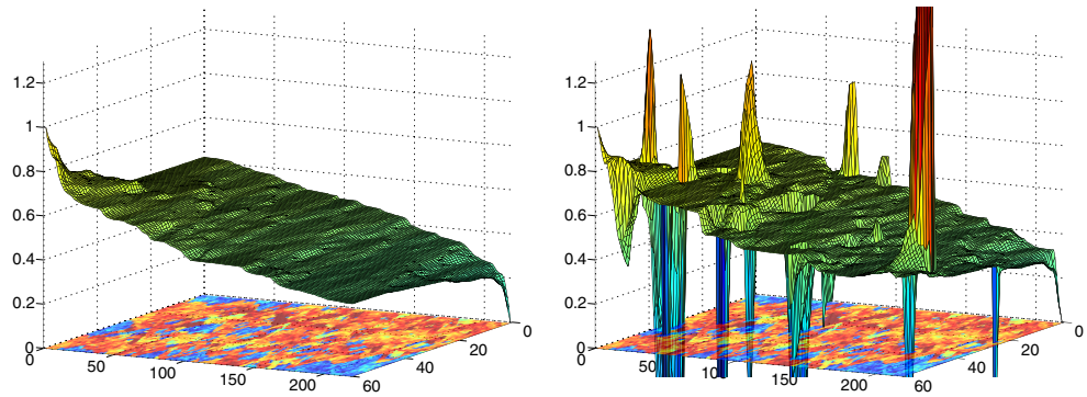
Fig. 7 Fine-scale reference (left) and MSFV (right) solutions for the SPE 10 bottom layer heterogeneous test case. There exist 220 \times 60 fine- and 20 \times 12 coarse- grid cells. Note that the MSFV superimposed solution (right) entails several non-physical peaks. The permeability field is also partly shown in the plots under the pressure solution
