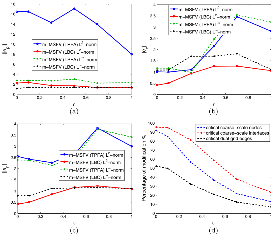
Fig. 20 Error measurements in pressure (a), velocity (b), residual (c) and computational complexity (d) with different threshold \varepsilon for the SPE 10 top layer with stretched grids
