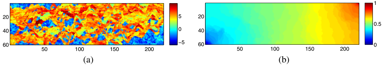
Fig. 10 Natural logarithm of the permeability (a) and fine-scale reference pressure (b) for the SPE 10 bottom layer
