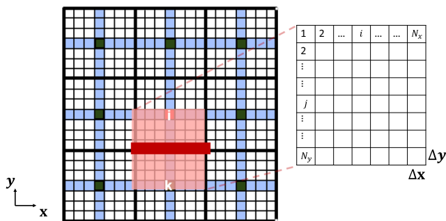
Fig. 8 Automatically detected critical interface (shown in bold red) where a_{ik}^c \not\leq 0 . The highlighted region with a pink rectangle shows the local domain, where the transmissibility is calculated using summation of harmonically averaged values to replace with a_{ik}^c and a_{ki}^c
