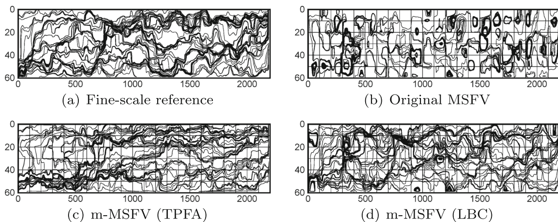
Fig. 22 Streamline plots based on velocity fields reconstructed by fine-scale reference, original and m-MSFV pressure solutions for the SPE 10 bottom layer with stretched grids. The coarse-scale grids are indicated by black lines
