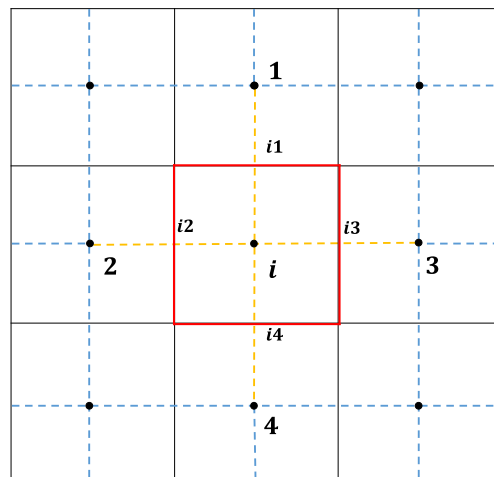
Fig. 9 Critical coarse node i and its neighboring faces F_{ij} (indicated by red solid lines) and edges E_{ij} (indicated by yellow dash lines), j = 1, 2, 3, 4 for 2D domain. The black lines indicate the coarse volumes
