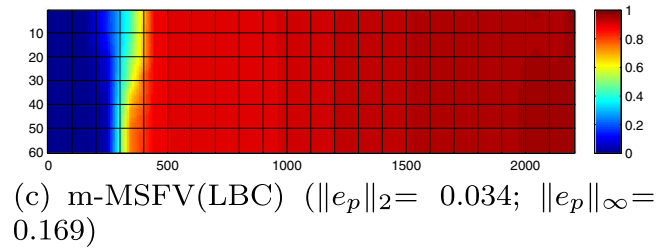
Fig. 17 Original MSFV and m-MSFV pressure solutions for the SPE 10 top layer with stretched grids, and the relative errors e_p
