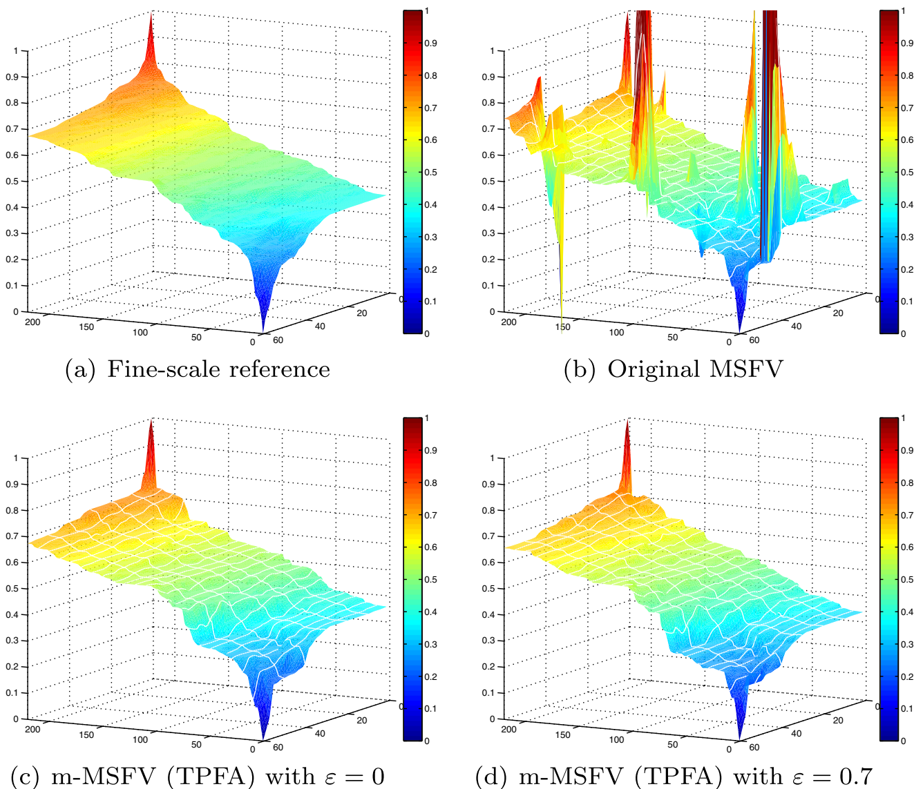
Fig. 14 Pressure surface plots for fine-scale reference (a), original MSFV (b), m-MSFV (TPFA) with \varepsilon = 0 (c) and \varepsilon = 0.7 (d), respectively
