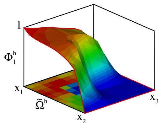
Fig. 2 Illustration of the basis function \Phi_1^h solved on dual-coarse cell \tilde{\Omega}^h subject to the reduced boundary condition. Note that the basis functions are always monotone and satisfy 0 \leq \Phi_k^h \leq 1 , provided that the mobility tensor \lambda is positive definite
