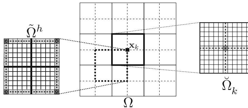
Fig. 1 Illustration of the MSFV primal- and dual-coarse grids imposed on the given 2D computational domain \Omega . The figure also shows the detail of a primal-coarse \tilde{\Omega}_k (coarse control volume) and a
