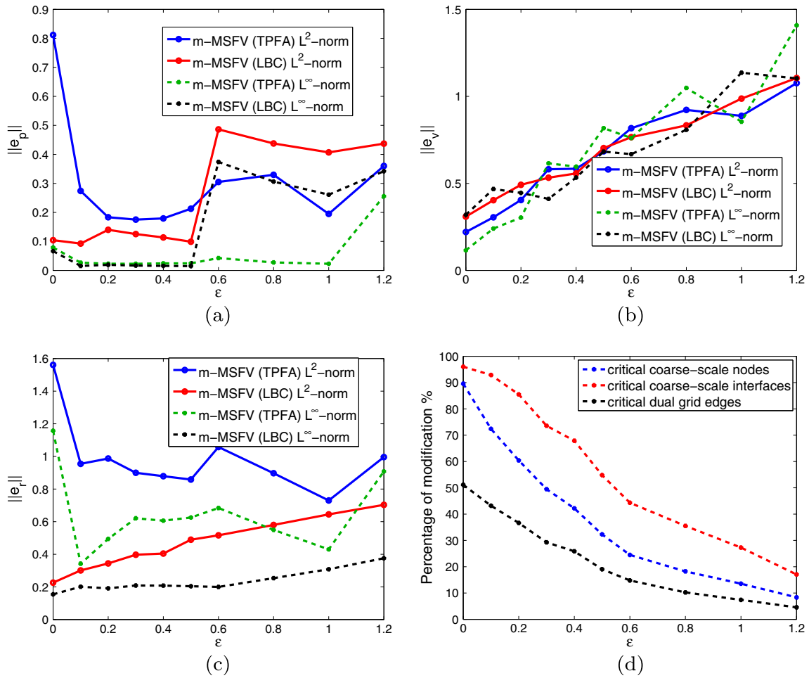
Fig. 23 Error measurements in pressure (a), velocity (b), residual (c), and computational complexity (d) with different threshold \varepsilon for the SPE 10 bottom layer with stretched grids
