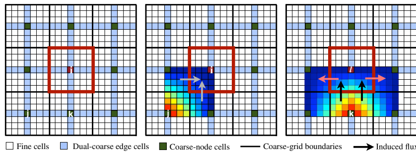
Fig. 3 (left): Illustration of a 3 \times 3 coarse- and 21 \times 21 fine- grid domain. The coarse cell i is highlighted in red, neighboring k and j on its South and South-West sides. Also shown are the induced fluxes by
