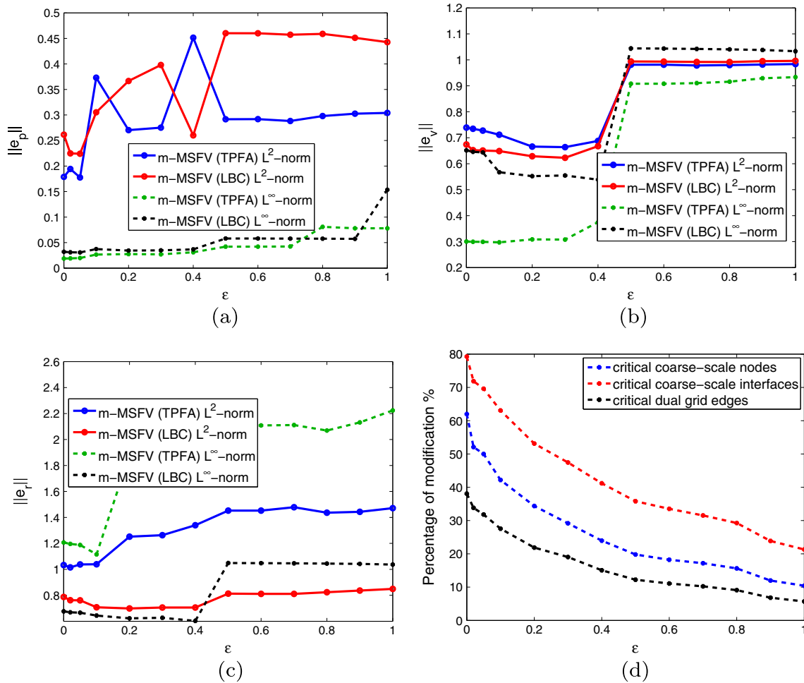
Fig. 15 Error measurements in pressure (a), velocity (b), residual (c), and the computational complexity (d) with different threshold \varepsilon for the SPE 10 bottom layer
