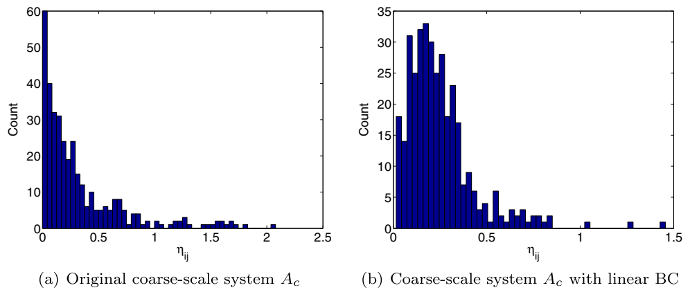
Fig. 19 Histogram of \eta_{ij} of the coarse-scale system A_c for original MSFV (a) and the reconstructed coarse-scale system for m-MSFV (LBC) (b), respectively, for the SPE 10 top layer with stretched grids. Note that m-MSFV (TPFA) eliminates all the positive indicators, therefore the histogram is not shown
