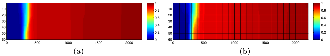
Fig. 24 Pressure distributions for fine-scale reference (a) and obtained by hybrid m-MSFV method (b) for the SPE 10 top layer with stretched grids, i.e., \Delta x = 10\Delta y
