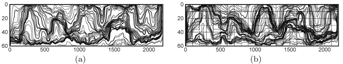
Fig. 25 Velocity distributions for fine-scale reference (a) and obtained by hybrid m-MSFV method (b) for the SPE 10 top layer with stretched grids, i.e., \Delta x = 10\Delta y
