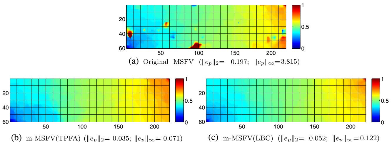
Fig. 11 Original MSFV and m-MSFV pressure solutions for the SPE 10 bottom layer, and the relative errors e_p . The coarse-scale grids are indicated by black lines
