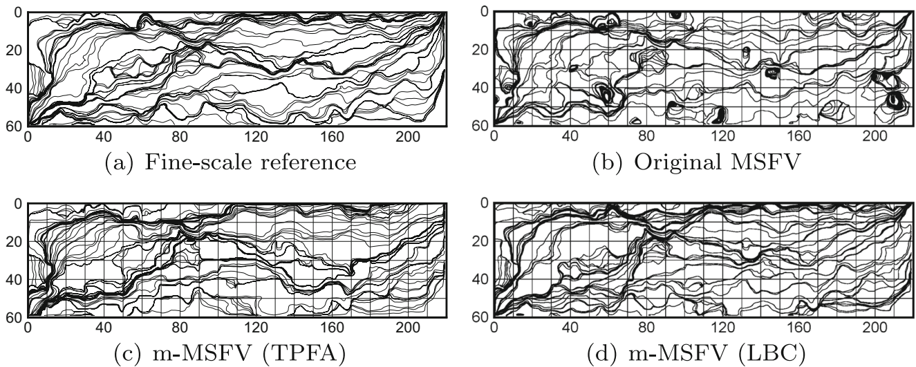
Fig. 12 Streamline plots based on velocity fields reconstructed by fine-scale reference, original and m-MSFV pressure solutions for the SPE 10 bottom layer. The coarse-scale grids are indicated by black lines
