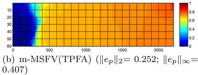
Fig. 17 Original MSFV and m-MSFV pressure solutions for the SPE 10 top layer with stretched grids, and the relative errors e_p
