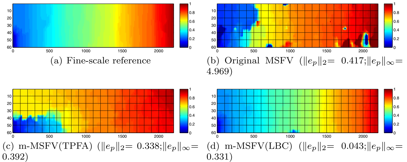
Fig. 21 Original MSFV and m-MSFV pressure solutions for the SPE 10 bottom layer with stretched grids, and the relative errors e_p
