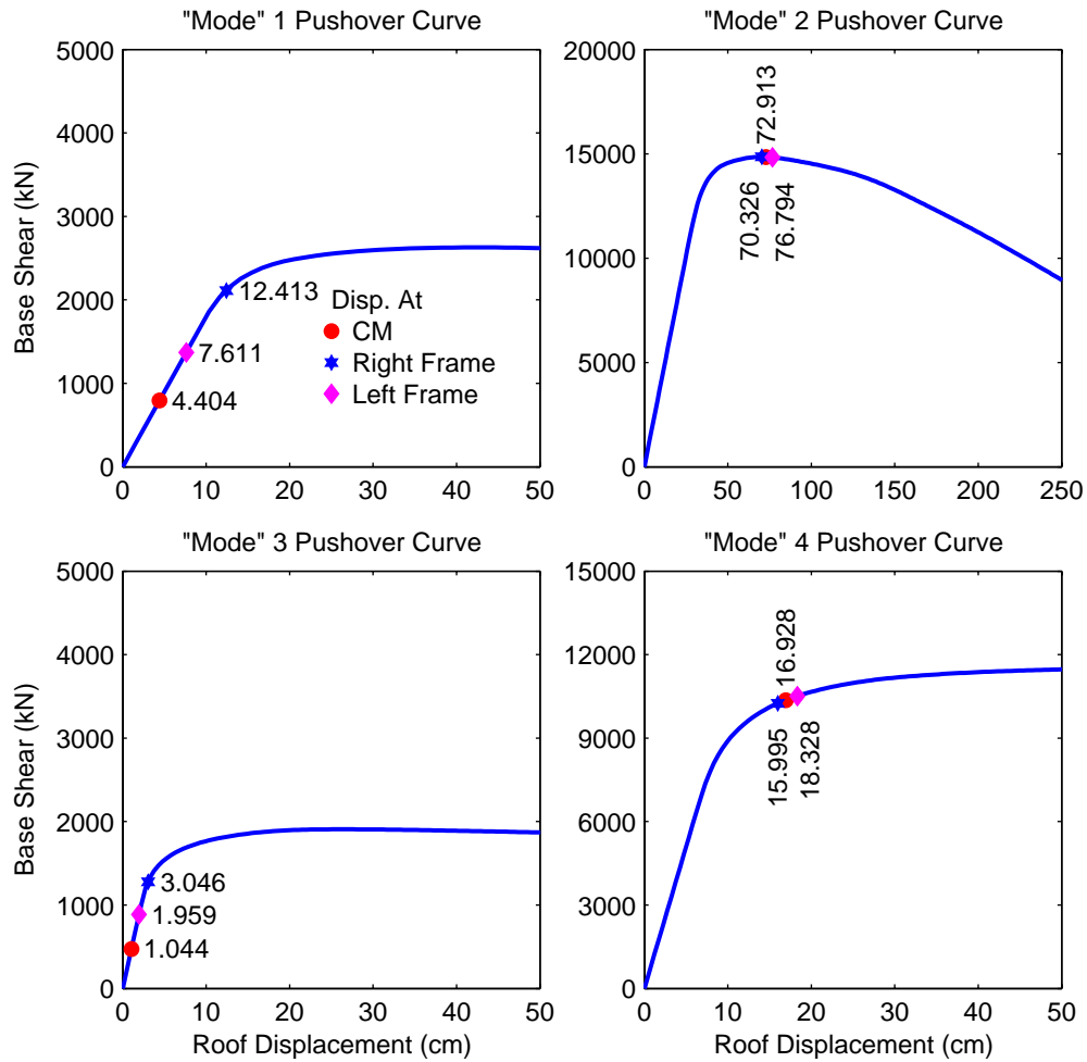
Figure 18. “Modal” pushover curves of unsymmetric-plan system U3 with target displacements at the roof CM in the UMRHA and MPA analyses identified; also identified are the peak roof displacement at the right and left frames.
