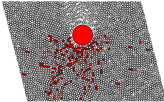
Fig. 23 Chains of particles forming beneath and to the side of the ball, adding upward force. A monolayer of particles in the xy plane is shown midway through the shear cycle, after the ball has fallen under gravity some distance. Small particles experiencing large-magnitude forces are coloured in red , indicating the chains of repulsion. The parameters used are k = 2 , f = 1 , in addition to those from Table 1. (Color figure online)
