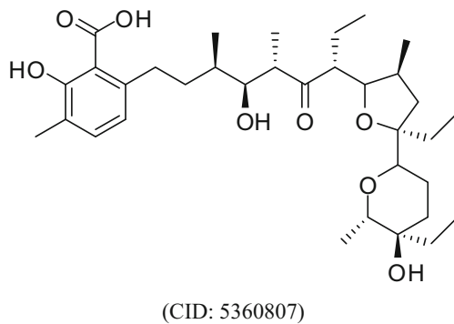
Fig. 1 Structure of lasalocid acid. The PubChem compound identifier (CID) for the compound is shown in parentheses
