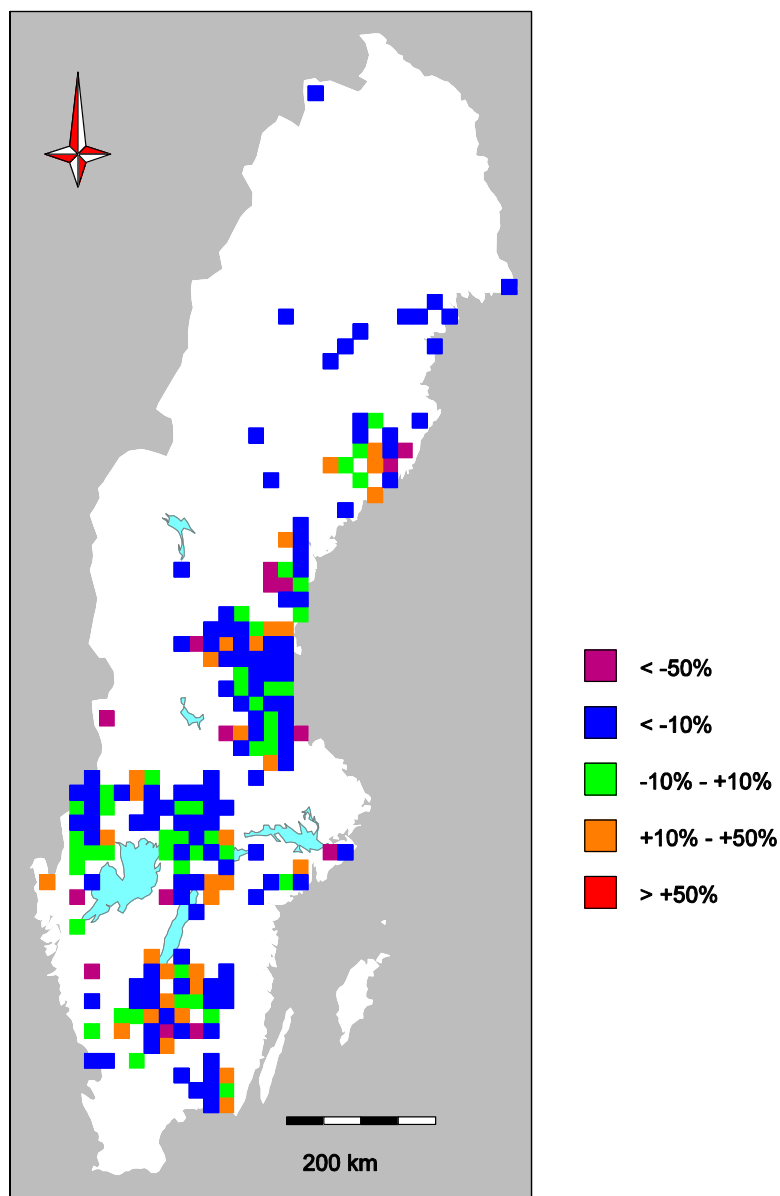
Fig. 4 Change in normalized (1-kg pike) total ww Hg concentrations based on 514 resampled lakes visited both 1965–1990 and 1991–2012. Colors show the mean change within 20 \times 20 km areas containing at least one resampled site. The average change was -20\%
