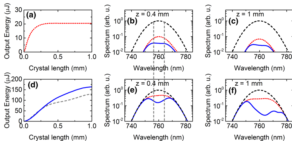
Fig. 7 Dynamics of mixing process for CP-DFG (a–c). a, d Idler power inside nonlinear crystal (GS) for compressed pump and signal (blue solid line: with intensity ratio optimization, gray dashed line: pump and signal with equal intensity). d–f Dynamics of CP-DFG
