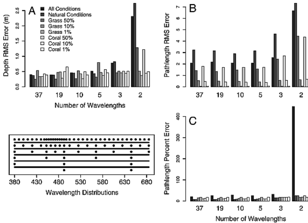
Figure 6. (a) RMS error of depth prediction from training on the year 2000 data and predicting the 2001 data for various numbers of spectral wavelengths used in the model. For all eight conditions, as little as three wavelengths from the spectral water-leaving radiance are needed for robust prediction of the depth of the bioluminescent layer. (b) RMS error of \tau prediction from training on the year 2000 data and predicting the 2001 data for various numbers of spectral wavelengths used in the model. Errors are not directly comparable because \tau also depends on the attenuation, which changed significantly between the eight conditions tested. (c) Path length errors as a percentage show that errors for all conditions are relatively low when more than five wavelengths are used in a neural net model. Errors increase slightly with three and two wavelengths in a neural net model in most conditions, but increase significantly with neural nets trained on all conditions. The bottom left panel shows wavelengths used in the reduction procedure. At each reduction step the number of wavelengths was reduced by \sim 50\% and alternate wavelengths were chosen. Enhanced EPS [311 KB]
