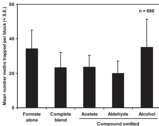
Fig. 5. M. gulosa field trial examining the relative attractiveness of highly isomerically pure (99% EE isomer) compounds in four component blend versus single deletions from that blend and the formate alone. Base blend consisted of 10:80:75:32 \mu\text{g} per septum (8 E ,10 E )-tetradecadienal, (8 E ,10 E )-tetradecadien-1-ol, (8 E ,10 E )-tetradecadien-1-yl formate, and (8 E ,10 E )-tetradecadien-1-yl acetate, respectively. Field trial was conducted at the Coachella Valley site from 18 to 28 July 2003. Treatments were not significantly different (two-way ANOVA: for treatment effect, F = 2.11 , df = 4, 24 , P = 0.13 ; for block effect, F = 34.29 , df = 4, 24 , P < 0.0001 ).
