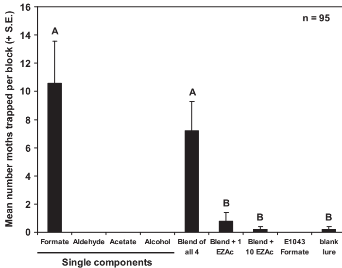
Fig. 7. M. gulosa field trial conducted in the Coachella Valley, comparing the attractiveness of lures containing single components to that of a blend of four components with and without 1 or 10 \mu\text{g} per septum 8E,10Z-14:Ac. Single components were tested at the 100 \mu\text{g} per septum dose, whereas the ratio in the four-component blend was 8:65:100:67 \mu\text{g} each of 8E,10E-14:Ald, 8E,10E-14:OH, 8E,10E-14:formate, and 8E,10E-14:Ac, respectively, per septum. Field trial conducted from 12 to 26 October 2006. Bars with different letters are significantly different (two-way ANOVA followed by Student–Newman–Keuls test, \alpha = 0.05 : for treatment effect, F = 14.89 , df = 4, 24 , P < 0.0001 ; for block effect, F = 1.02 , df = 4, 24 , P = 0.43 ).
