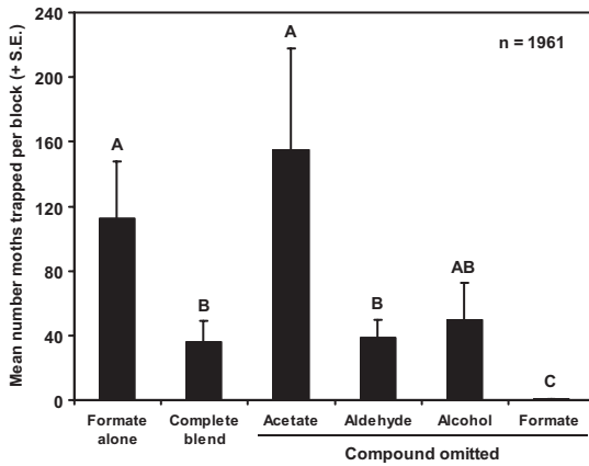
Fig. 4. M. gulosa field trial examining the relative attractiveness of a four component blend versus single deletions from that blend and (8 E ,10 E )-tetradecadien-1-yl formate as a single component. Base blend consisted of 10:80:75:32 \mu\text{g} per septum (8 E ,10 E )-tetradecadienal, (8 E ,10 E )-tetradecadien-1-ol, (8 E ,10 E )-tetradecadien-1-yl formate, and isomerically impure (94% EE ) (8 E ,10 E )-tetradecadien-1-yl acetate, respectively. Field trial was conducted at the Coachella Valley site from 3 to 18 July 2003. Treatments with different letters are significantly different (two-way ANOVA followed by Student–Newman–Keuls test, \alpha = 0.05 : for treatment effect, F = 4.45 , df = 4, 24 , P = 0.013 ; for block effect, F = 8.03 , df = 4, 24 , P = 0.0009 ).
