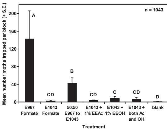
Fig. 8. Field trial conducted in the San Joaquin Valley comparing attractiveness of 8E,10E-14:formate lots synthesized by different routes. Single components were tested at the 100 \mu\text{g} per septum dose. Field trial conducted from 26 October to 16 November 2006. Bars with different letters are significantly different (two-way ANOVA followed by Student–Newman–Keuls test, \alpha = 0.05 : for treatment effect, F = 15.44 , df = 6, 34 , P < 0.0001 ; for block effect, F = 1.17 , df = 4, 34 , P = 0.35 ).
