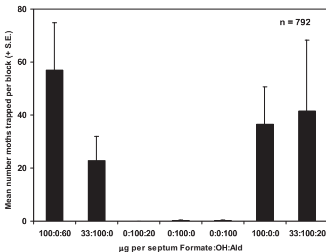
Fig. 3. M. gulosa field trial testing (8 E ,10 E )-tetradecadienal, (8 E ,10 E )-tetradecadien-1-ol, and (8 E ,10 E )-tetradecadien-1-yl formate, conducted at the Coachella Valley site 21 June-27, 2002. Treatments capturing more than a single insect were not significantly different (two-way ANOVA: for treatment effect, F = 1.96 , df = 3, 19 , P = 0.17 ; for block effect, F = 7.16 , df = 4, 19 , P = 0.004 ).
