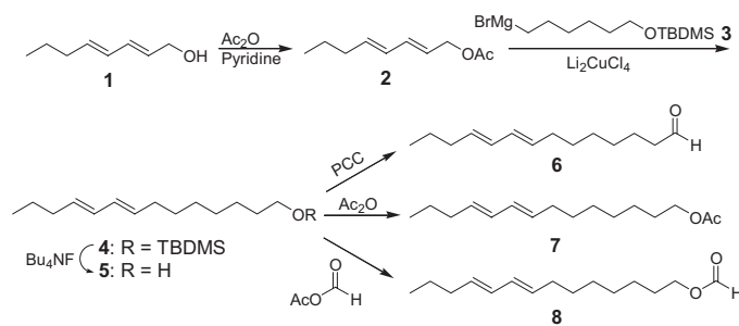
Fig. 1. Synthesis of the possible pheromone components 8E,10E-14:OH, 8E,10E-14:Ald, 8E,10E-14:formate, and 8E,10E-14:Ac.
