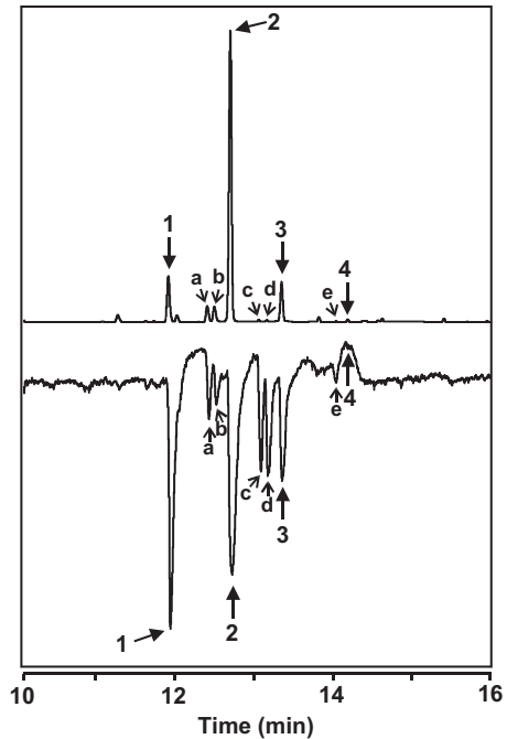
Fig. 2. Coupled GC-EAD traces from an SPME collection of volatiles from three female M. gulosa over a single night. Column: DB-5, 30 m by 0.25 mm i.d. by 0.25- \mu\text{m} film, temperature program 100°C/1 min and then 10°C/min to 250°C for 20 min. Peak 1, (8E,10E)-tetradecadienal; peak 2, (8E,10E)-tetradecadien-1-ol; peak 3, (8E,10E)-tetradecadien-1-yl formate; peak 4, (8E,10E)-tetradecadien-1-yl acetate; peaks a and b, (8Z,10E)- and (8E,10Z)-tetradecadien-1-ol, respectively; peaks c and d, (8Z,10E)- and (8E,10Z)-tetradecadien-1-yl formate, respectively; and peak e, (8E,10Z)-tetradecadien-1-yl acetate.
