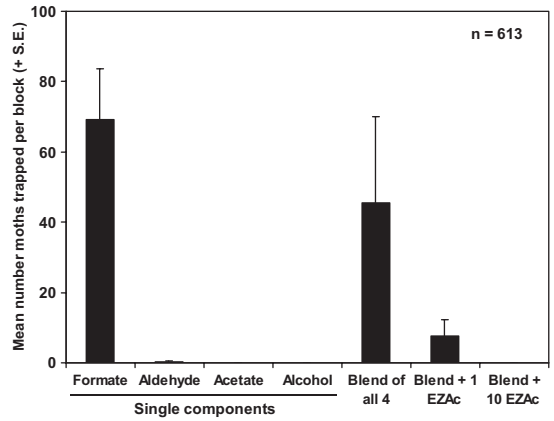
Fig. 6. M. gulosa field trial conducted in the San Joaquin Valley, comparing the attractiveness of lures containing a blend of 8 E ,10 E -14:Ald, 8 E ,10 E -14:OH, 8 E ,10 E -14:formate, and 8 E ,10 E -14:Ac (8:65:100:67 \mu\text{g} per septum, respectively), alone or in combination with a 1 or 10 \mu\text{g} per septum dose of 8 E ,10 Z -14:Ac, and single component lures with 100 \mu\text{g} per septum of each of the compounds (excluding the 8 E ,10 Z -14:Ac). Field trial conducted from 14 to 28 September 2006. Bars with different letters are significantly different (two-way ANOVA on \log_{10}(x + 1) -transformed data followed by Student–Newman–Keuls test, \alpha = 0.05 : for treatment effect, F = 11.48 , df = 3, 19 , P = 0.0008 ; for block effect, F = 3.56 , df = 4, 19 , P = 0.039 ).
