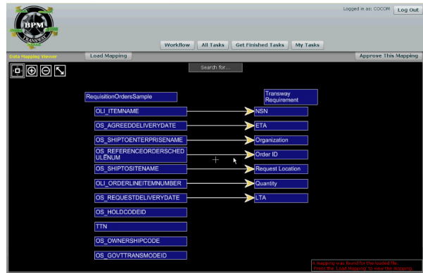
Figure 4. The graphical mapping tool.
