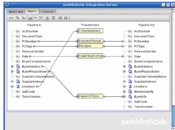
Figure 1. WebMethods Integration Server, using a graphical mapping tool. Source: http://www1.webmethods.com/images/products/screenshots/wm_ESP_BI_2.jpg
