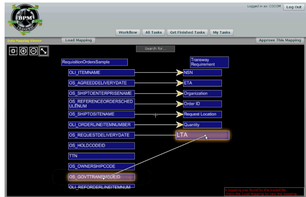
Figure 5. A mapping is suggested automatically by IMT.
