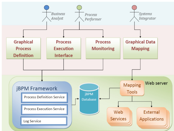
Figure 3. The Integration Platform
