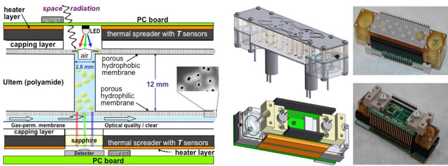
Fig. 45 Left: Cross-sectional view of a single 75- \mu L microwell and the associated fluid delivery, thermal control, and optical measurement components. Right: Four different views (solid model at left , photographs at right ) of one of three bioblocks included in the O/OREOS-SESLO payload. The two solenoid valves protrude down from the block ( upper left ); reservoirs are the elliptical structures at both ends of the block; heater is orange; radiation-sensitive FET (RadFET), which measured integrated radiation dose at two locations in the SESLO payload cubes, is a black dot near the center of the bottom left
