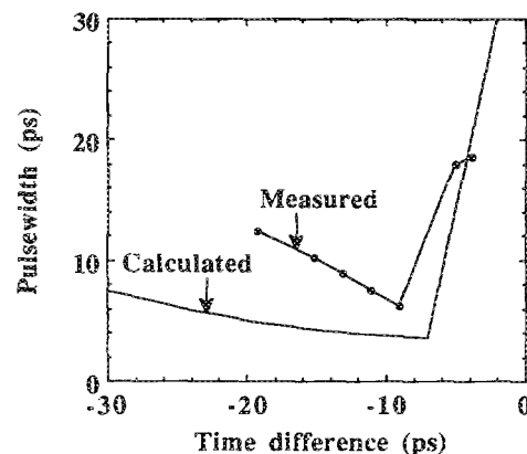
FIG. 5. Optical pulse width vs arrival time difference between the electrical and optical pulses at the gain region.
