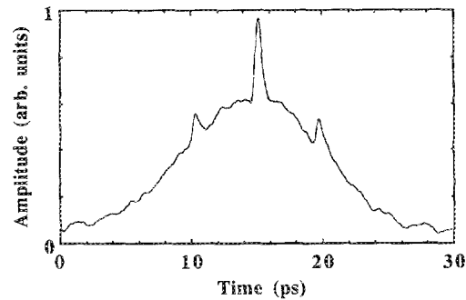
FIG. 4. Second-harmonic trace of a 1.5 GHz ( n = 3 , m = 10 ) repetition rate output pulse. The optical pulse FWHM is 8 ps assuming a hyperbolic secant squared pulse shape.
