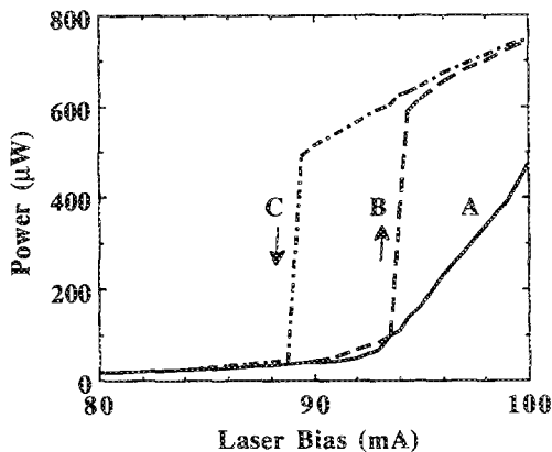
FIG. 3. Light output vs current for the self-mode-locked laser. Trace A shows the measurement without optical to electrical converter feedback. Traces B and C show the measurement with O/E converter feedback.
