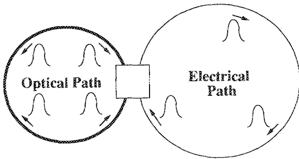
FIG. 2. Circulating electrical and optical pulses in the laser for the case where the electrical path delay is 1.5 times the optical path delay ( n = 2 , m = 3 ).
