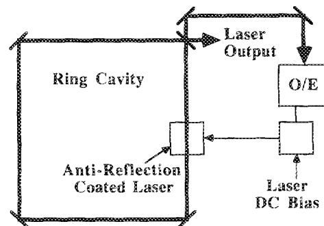
FIG. 1. Experimental setup for self-mode-locking. There are two feedback loops: one for the optical signal, and one for the optical to electrical converter.
