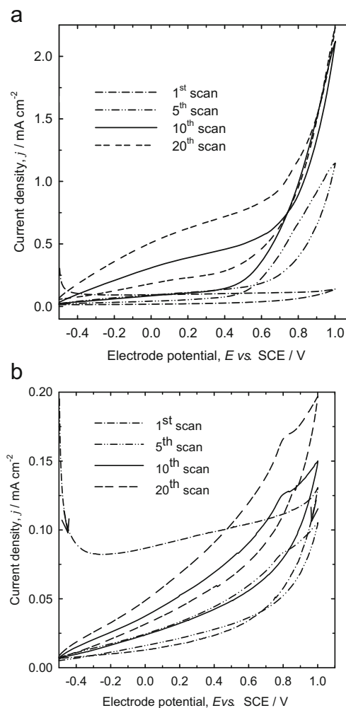
Fig. 3 Cyclic voltammetry for an AZ31 Mg alloy for 20 cycles at a potential sweep rate of 20 mV s ^{-1} in a solution containing 0.5 mol dm ^{-3} SA, 0.5 mol dm ^{-3} Py with a 10 \times 10^{-3} mol dm ^{-3} IBU and b 50 \times 10^{-3} mol dm ^{-3} IBU. The electrode was immersed in the solution for 10 min before starting
