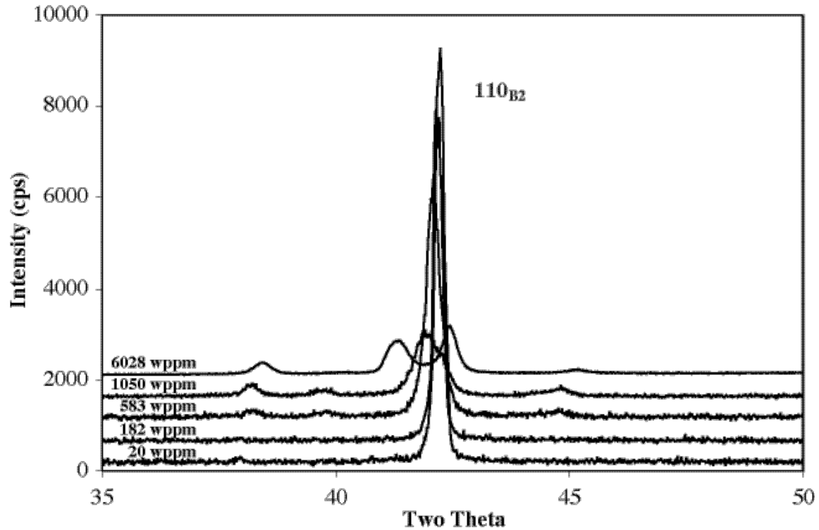
Figure 1: X-ray diffraction patterns of annealed and hydrogenated Ti_{49.2}Ni_{50.8} wires. Note the dramatic change in position and intensity of the diffraction peaks near 42^\circ 2\theta with increased hydrogen.
