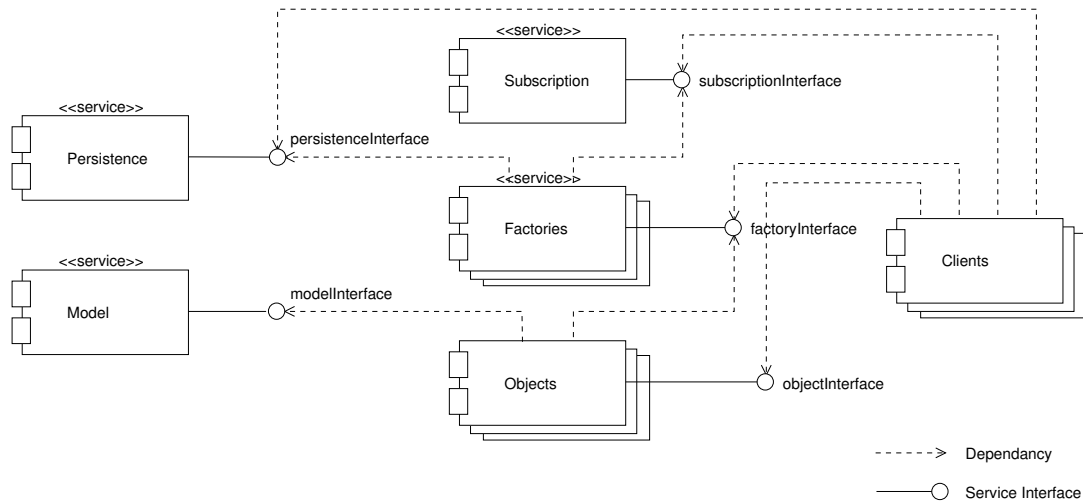
Figure 1.3: ICDM Services
