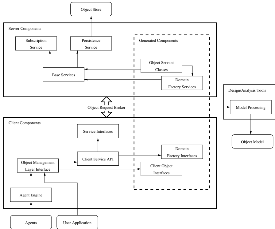
Figure 1.2: ICDM Component Diagram
