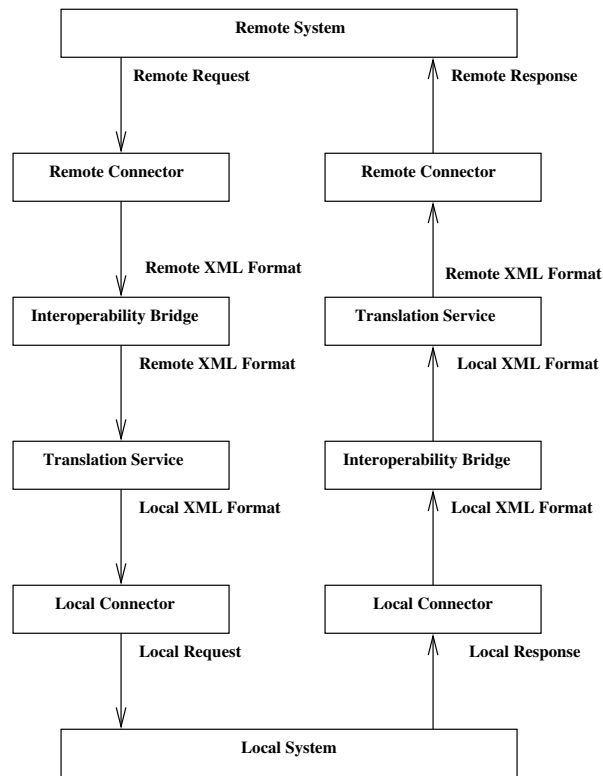
Figure 9.2: Request/Response path
