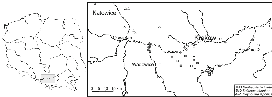
Fig. 1 Location of the study area and 48 sites within (gray symbols) and outside valleys (white symbols). Within each site, two plots (invasive vs. native) were localized
