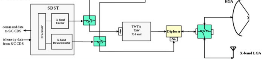
Fig. 24 Block diagram for the AVIATR telecommunications systems
