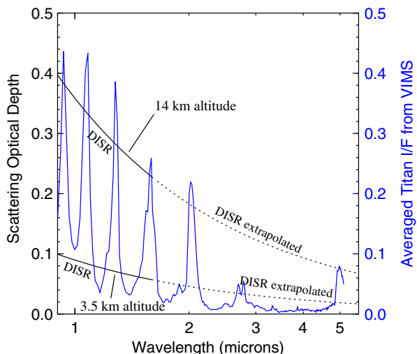
Fig. 29 Here we plot the normal scattering optical depth of Titan’s atmosphere (black, with scale at left ) from an altitude of 14 km ( top, black ) and 3.5 km ( bottom, black ). These values come from the DISR parameterization, and are extrapolated beyond the DISR wavelength cutoff at 1.6 \mu\text{m} . Also shown is a typical exoatmospheric Titan spectrum from VIMS (blue, with scale at right ); the atmospheric windows show up as relative peaks in the VIMS spectrum
