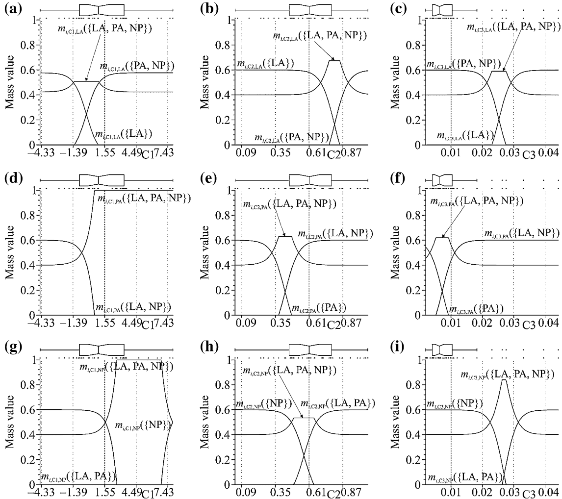
FIGURE 3. NCaRBS induced graphical representation of the mass values making up the constituent BOEs, m_{i,C1,LA}(\cdot) , m_{i,C2,PA}(\cdot) and m_{i,C3,PA}(\cdot) , relating to C1 (pelvic obliquity, degrees), C2 (frontal moment, Nm/kg) and C3 (frontal power, W/kg) measured at 30 s into single-leg stance, and the evidence towards the surgery types, LA, PA, and NP and against \{-LA\} = \{PA, NP\} , \{-PA\} = \{LA, NP\} and \{-NP\} = \{LA, PA\} and ignorance \{LA, PA, NP\} .
