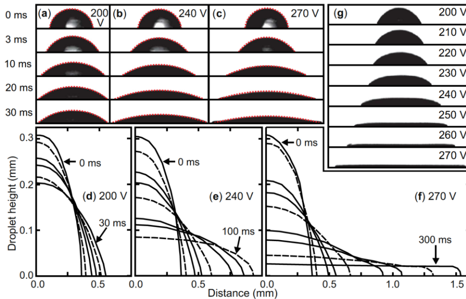
Figure 2. Dynamic drop shape profiles at different spreading voltages. Panels (a) – (c) show actual drop shape profiles viewed from the y -direction and panels (d) – (f) show digitised drop shape profiles. The profiles are shown as a function of time after a constant amplitude sine wave voltage (10 kHz) is applied to the electrodes: (a) and (d) just below the threshold voltage (200 V, V/V_{Th} = 0.87 ); (b) and (e) just above the threshold voltage (240 V, V/V_{Th} = 1.04 ); and (c) and (f) further above the threshold voltage (270 V, V/V_{Th} = 1.17 ). In panels (d) – (f) digitised profiles are shown at times 0, 1 ms (dashed), 3 ms, 5 ms, 10 ms (dashed), 30 ms, 50 ms, 100 ms (dashed) and 300 ms. The red dashed lines shown in panels (a) – (c) are fits to circular arcs. Panel (g) shows equilibrium (long time limit) droplet shapes viewed from the y -direction for a range of different spreading voltages from 200 V to 270 V. The vertical scale in panel (g) is expanded by a factor of 2 compared to the horizontal scale so that the spread film at 270 V can be clearly seen.
