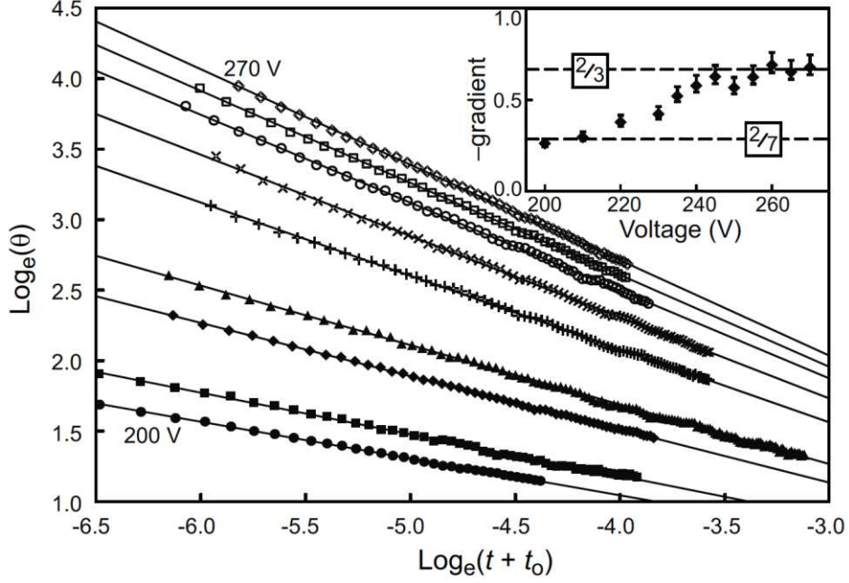
Figure 4. Power law spreading ( V \sim V_{\text{Th}} ) and superspreading ( V > V_{\text{Th}} ) of stripes on interdigital electrodes showing dynamic contact angle \theta \propto 1/(t+t_0)^n . Data are shown for applied voltages of 200 V (filled circle), 210 V (filled square), 220 V (filled diamond), 230 V (filled triangle), 235 V (plus), 240 V (cross), 255 V (open circle), 265 V (open square) and 270 V (open diamond). The time is denoted by t , and t_0 is a constant at each voltage. For clarity, all curves have been offset to pass through the origin. Inset: n is close to 2/7 at voltages just below V_{\text{Th}} , rising to 2/3 as the voltage is increased above V_{\text{Th}} .
