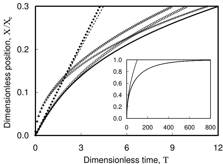
Figure 4. Comparison of approximate analytical solutions for Bousanquet (ooo), visco-gravitational (+++), Lucas-Washburn (AAA), inertial (●●●) and inertial with gravity correction (- - -) to the exact numerical solution (solid line) for G=0.1 and \varphi=90^\circ . The capillary rise height X is shown as a fraction of the equilibrium rise height, X_e . The inset shows the long time behaviour for the exact solution and the Bousanquet solution. On this scale the visco-inertial cannot be distinguished from the exact solution and the Lucas-Washburn approximation cannot be distinguished from the Bousanquet solution on the longer time scale.
