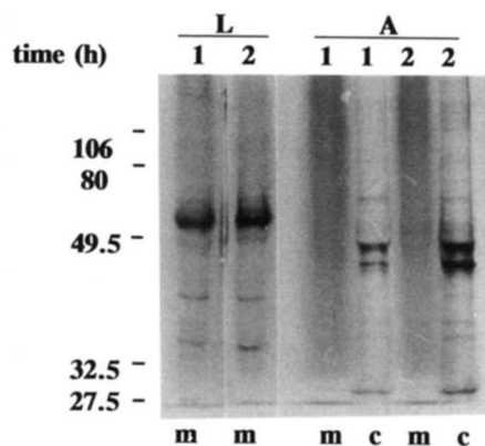
Fig. 6. Pulse-labeling of adrenocortical cells and liver cells with [ 35 S]methionine. Freshly isolated liver parenchymal cells (L) and adrenocortical cells (A) were incubated for the indicated time with [ 35 S]methionine. After pulse-labeling, the cell-free media (m) and cell lysates (c) were incubated with polyclonal anti-HL IgGs immobilized on Sepharose beads. The immunoabsorbed proteins were separated by SDS-PAGE on a 10% gel and visualized by fluorography. The positions of the pre-stained molecular weight markers are indicated.
