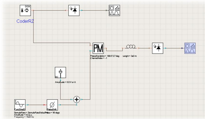
Figure 3-15: Numerical Simulation Setup (VPI Transmission Maker): RZ input pulses
