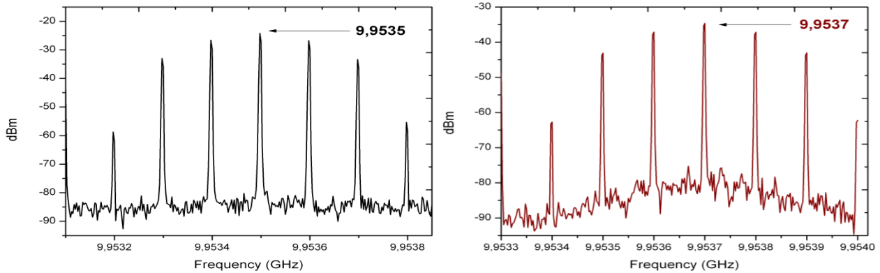
(a) input signal ( f = 9.9535 \text{ GHz} ) (b) output synchronized signal ( f_L = 9.9537 \text{ GHz} )
