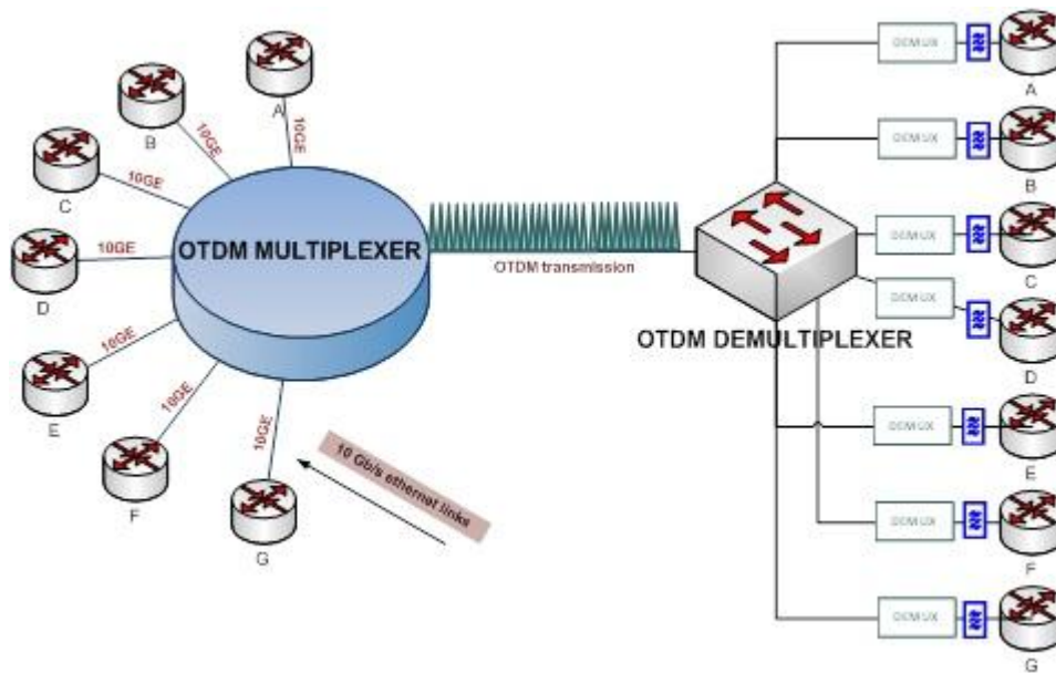
Figure 1-1: OTDM system multiplexing 10GE input frames
