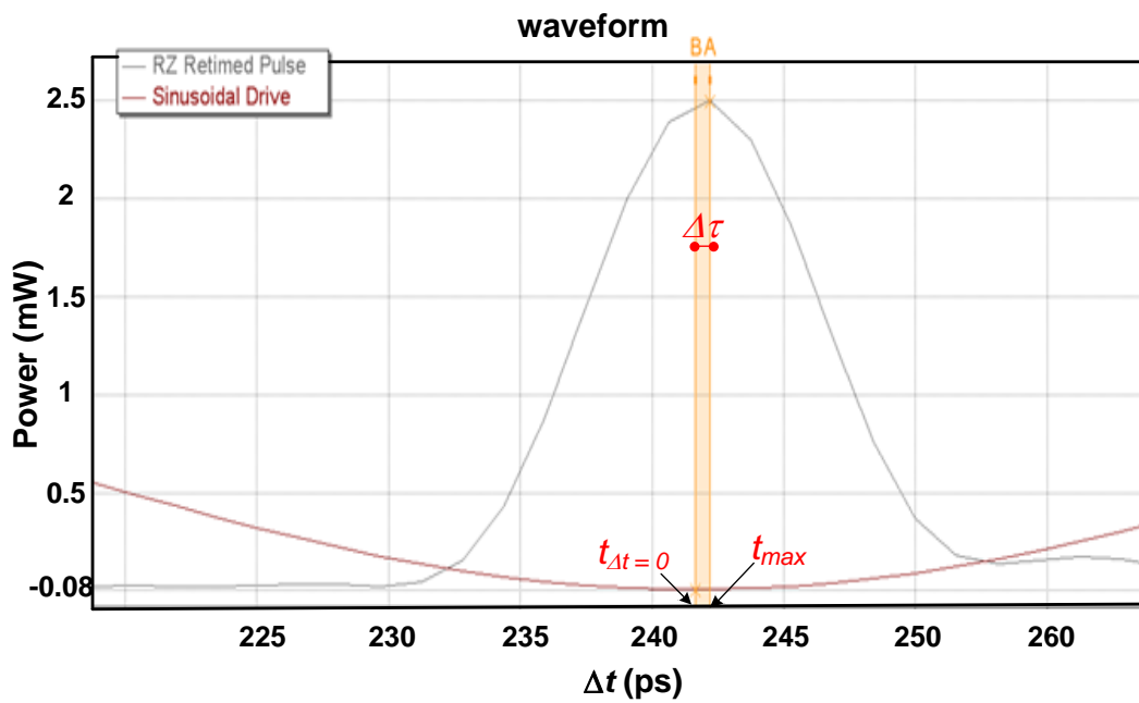
Figure 3-11: \Delta\tau definition: waveforms for (a) output RZ signal, and (b) sinusoidal clock ( \Delta t = 0.1 T_L )
