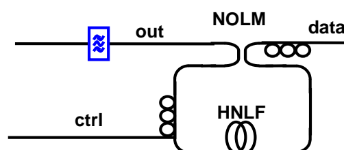
Figure 5-2: OTDM Demultiplexing
