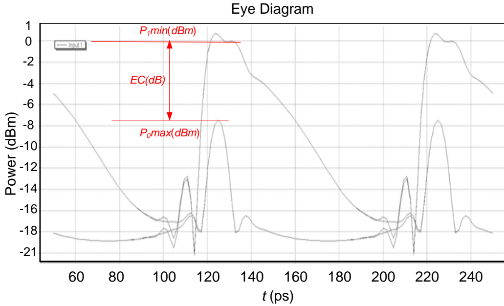
Figure 3-10: Eye Contrast Ratio ( \Delta t = T_L/4 )
