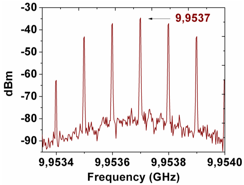
(a) generated 10GE frame pulses
