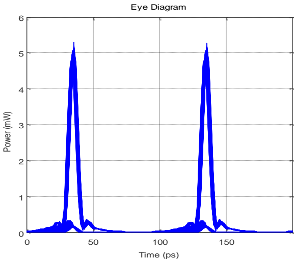
Figure 4-6: Eye diagram (oscilloscope triggered with local clock, f_L = 10.001 GHz)
