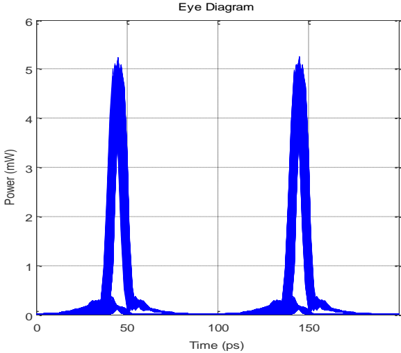
Figure 4-9: Eye diagram (oscilloscope triggered with local clock, f_L = 10.001 GHz)
