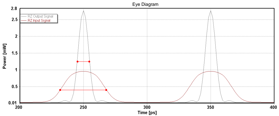
Figure 3-13: FWHM definition: eye-diagram for output RZ signal ( \Delta t = 0 )
