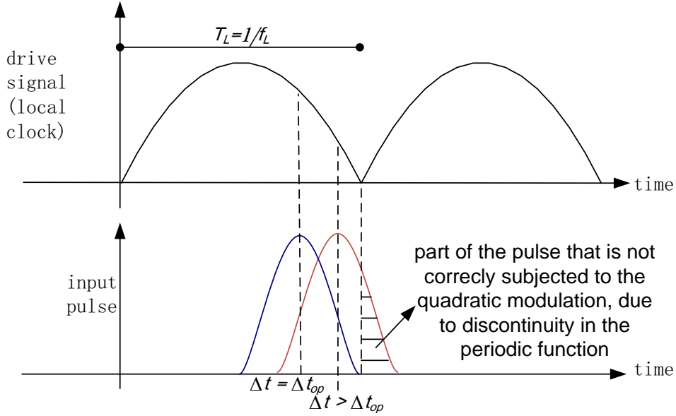
Figure 3-5: Operational range of a time-lens with periodic quadratic phase modulation
