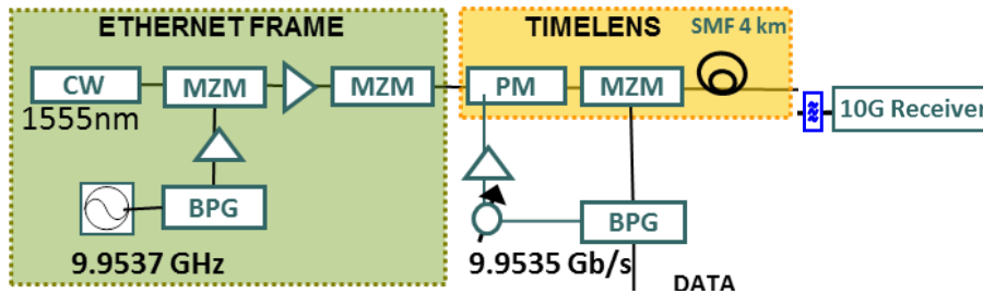
Figure 4-16: Laboratory SETUP [31]
