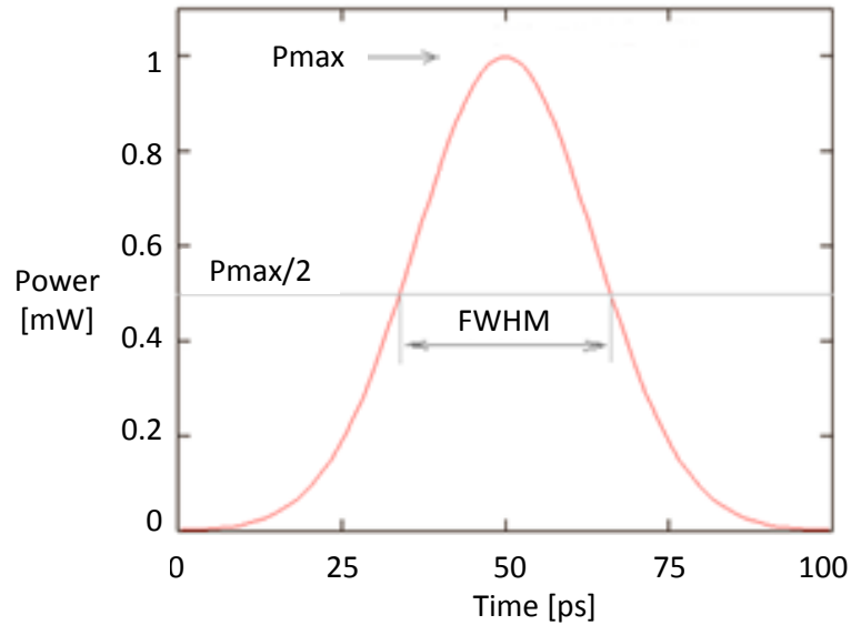
Figure 3-12: FWHM definition
