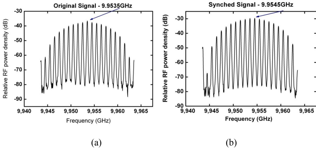
Figure 4-14: Electrical spectrum: (a) original and (b) synchronized signal
