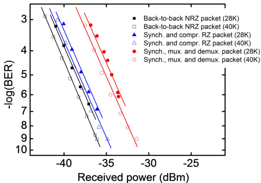
Figure 5-8: BER measurements
