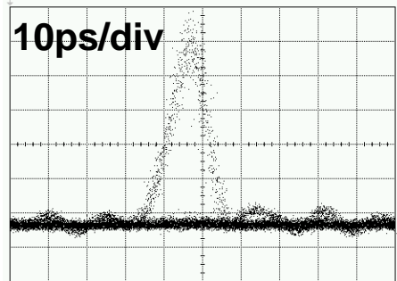
(b) 40 Kbit sized frame ( \Delta f = 100 kHz)
