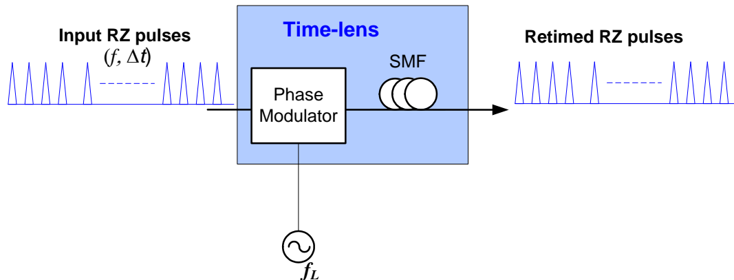
Figure 3-3: Time-lens used for Retiming of RZ input pulses
