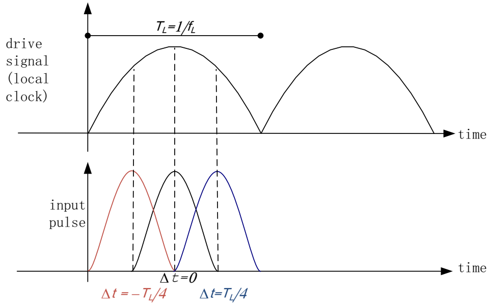
Figure 3-4: Time-misalignment between RZ input pulses and parabolic local clock
