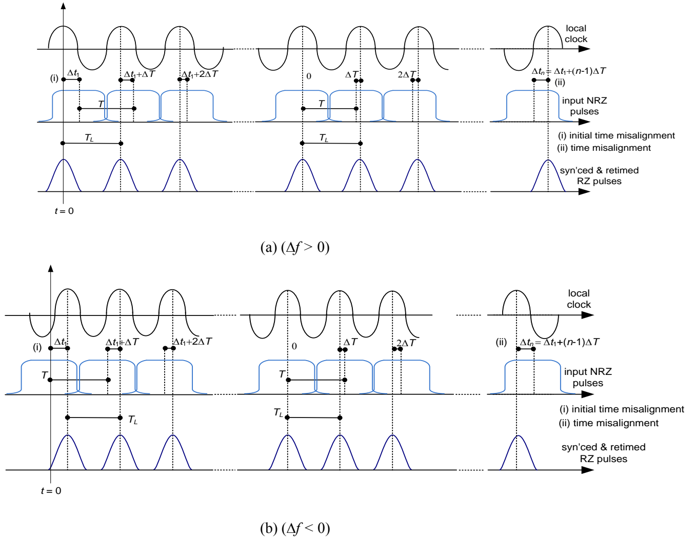
Figure 4-2: Operational principle of synchronization, retiming and format-conversion unit
