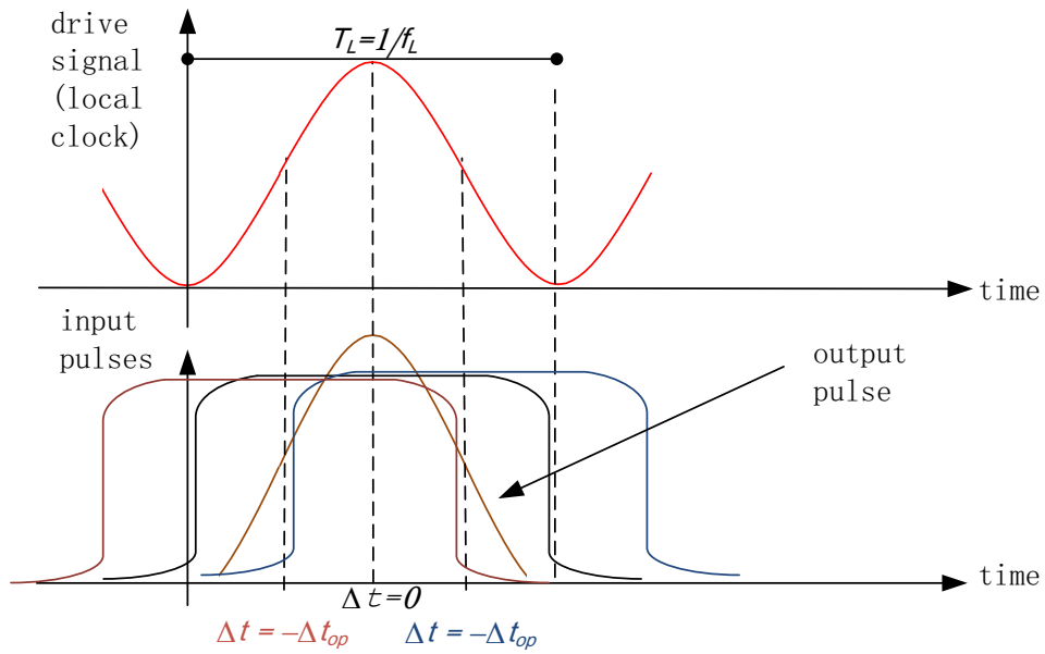
Figure 3-2: Time-misalignment of NRZ input pulses and MZM sinusoidal driving signal
