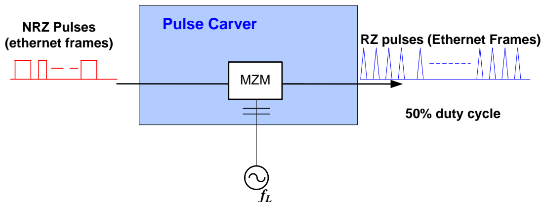
Figure 3-1: Pulse carver (MZM)
