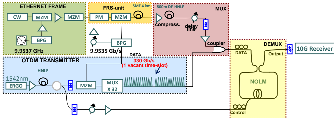
Figure 5-3: Laboratory experiment setup
