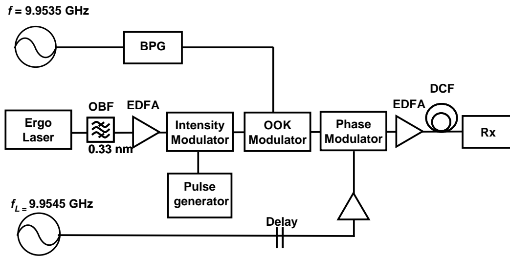
Figure 4-12: Experimental set-up to realize a FRS-unit.
