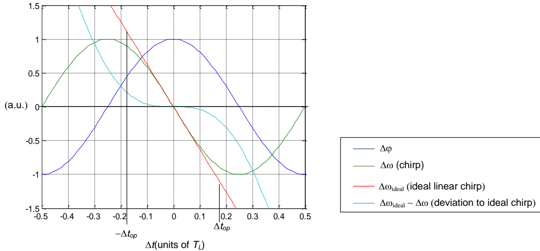
Figure 3-6: Ideal quadratic chirp vs. sinusoidal chirp
