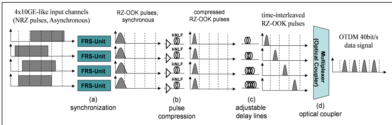
Figure 5-1: OTDM Multiplexing
