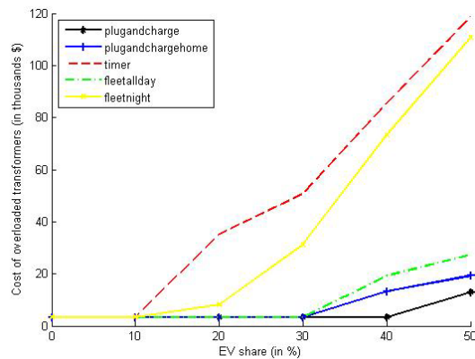
Figure 10 Replacement cost of overloaded transformers with different EV penetration levels and 3 Phase charging
