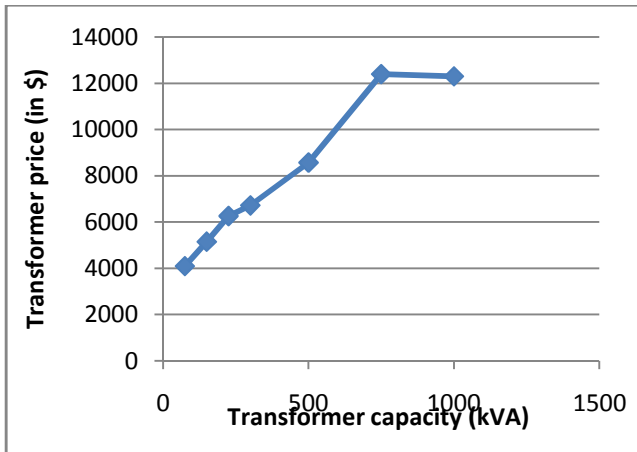
Figure 2 Distribution of transformer cost versus its capacity
