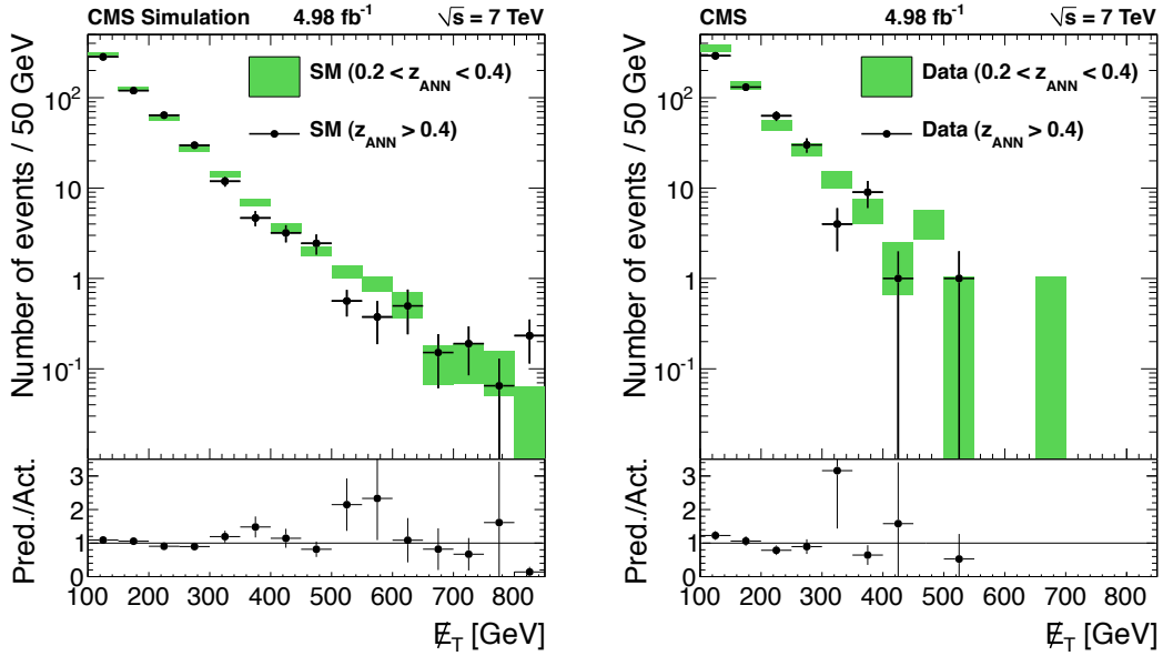
Figure 12: The E_T distributions of events in the z_{ANN} signal region (solid circles) and sideband (green bars) for simulated SM (left) and data (right) events. The distributions are normalized in the E_T sideband, 150 < E_T < 350 GeV (regions A and C for the two distributions respectively). The rightmost histogram bin includes overflow. The small lower plots show the ratio of normalized sideband to signal yields.
