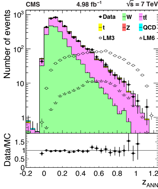
Figure 10: The z_{\text{ANN}} distribution of the data (solid circles) and simulated SM (stacked shaded histograms), LM3 (open circles), and LM6 (open triangles) events, after preselection. The small plot beneath shows the ratio of data to simulated SM yields.
