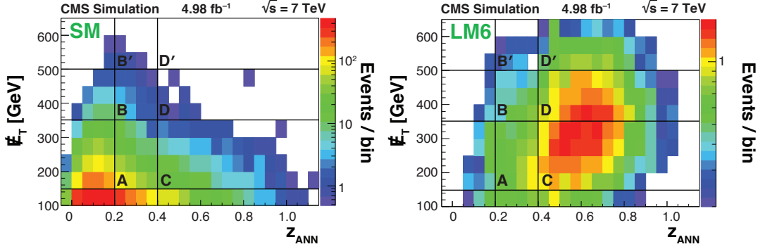
Figure 11: The yields of simulated SM (left) and LM6 (right) events in the E_T versus z_{ANN} plane. The regions D and D' are the low- E_T and high- E_T signal regions. The sideband regions are also indicated.
