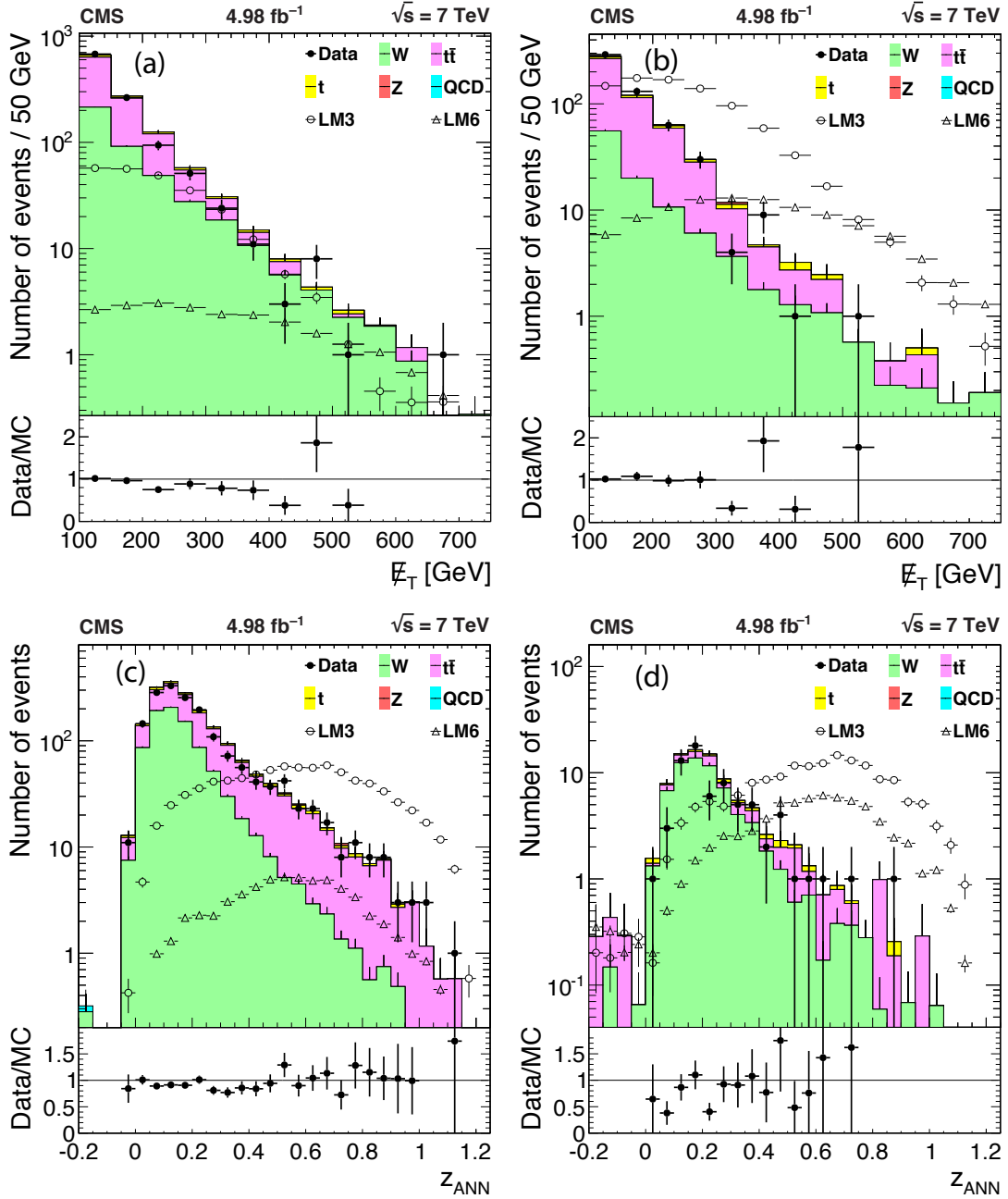
Figure 13: Distributions of E_T for (a) 0.2 < z_{ANN} < 0.4 and (b) z_{ANN} > 0.4 , and distributions of z_{ANN} for (c) 150 < E_T < 350 \text{ GeV} and (d) E_T > 350 \text{ GeV} . The samples shown are data (solid circles), simulated SM (stacked shaded histograms), LM3 (open circles), and LM6 (open triangles) events. The small plot beneath each distribution shows the ratio of data to simulated SM yields.
