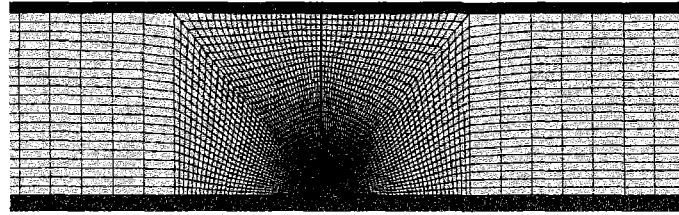
Fig. 3. Crack propagation from notch edge using CZM
