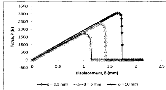
Fig. 4: Typical load-displacement plot implementing CZM approach of GFRP (0/90/±45) s lay-up
