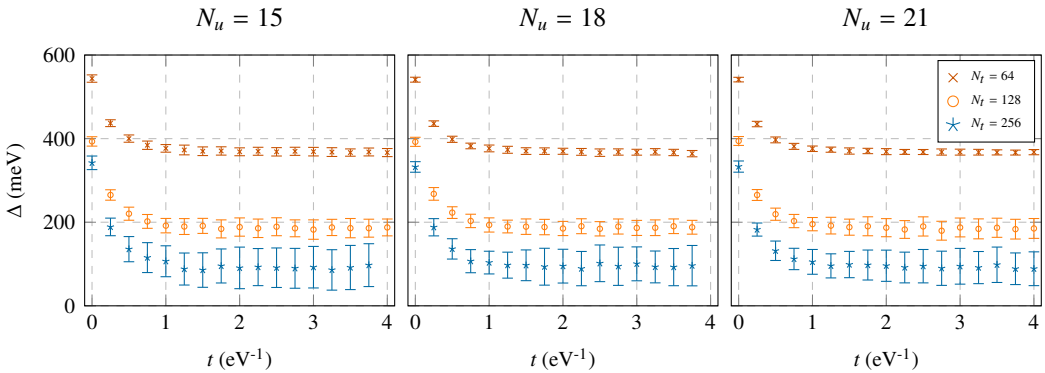
Figure 3. Value of the gap determined from the effective mass at the Dirac point with coupling U/\kappa = 1 and \beta = 8 \text{ eV}^{-1} for N_u = 15, 18, 21 and N_t = 64, 128, 256 . Results are nearly independent in N_u for this (weak) value of the coupling, but demonstrate strong dependence on N_t .
