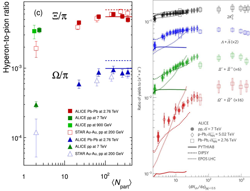
Figure 4. Left: the \Xi^-/\pi and \Omega/\pi ratios in pp and AA collisions as a function of \langle N_{part} \rangle [5]. The lines correspond to statistical model predictions (solid line [9], dashed line [10]). Right: the yield ratios of strange particles and pions measured in pp, pA and AA collisions at the LHC as a function of dN_{ch}/d\eta [11].
