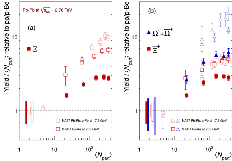
Figure 1. The enhancement factors for multi-strange (anti-)particles as a function of the number of participants \langle N_{part} \rangle as measured at the SPS [3], RHIC [4] and LHC [5].
