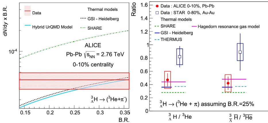
Figure 8. Left: the {}^3_{\Lambda}\text{H} yield as measured at the LHC in comparison to several model predictions [27]. Right: the {}^3_{\Lambda}\text{H}/{}^3\text{He} and {}^3_{\Lambda}\text{H}/{}^3\text{He} ratios measured at RHIC and LHC in comparison to statistical model predictions [27].
