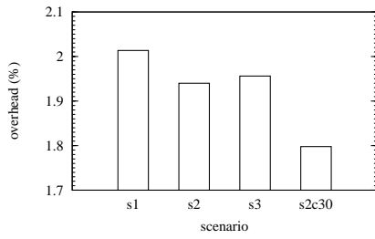
Figure 4.9: Overhead without DHT/DT
