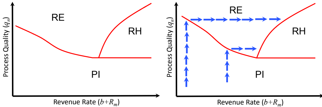
Figure 2 Optimal policy under Assumptions 1–3.
