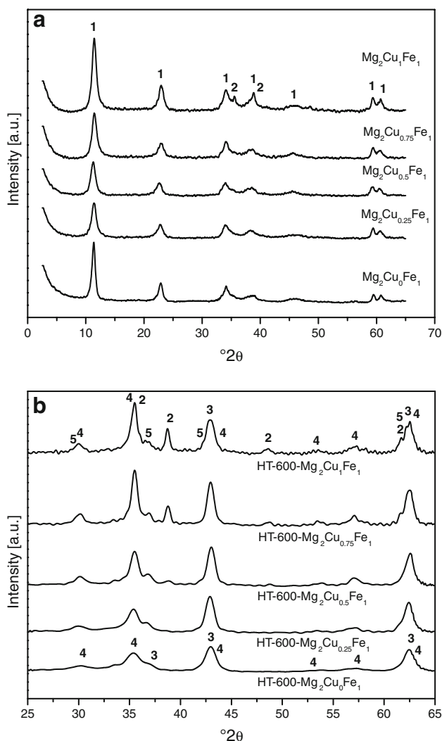
Fig. 1 X-ray diffraction patterns for hydrotalcite-like catalysts' precursors (a) and mixed metal oxide catalysts (b); 1—hydrotalcite, 2—tenorite, CuO, 3—periclase, MgO, 4—magnesioferrite, MgFe_2O_4 , 5—cuprite, Cu_2O
