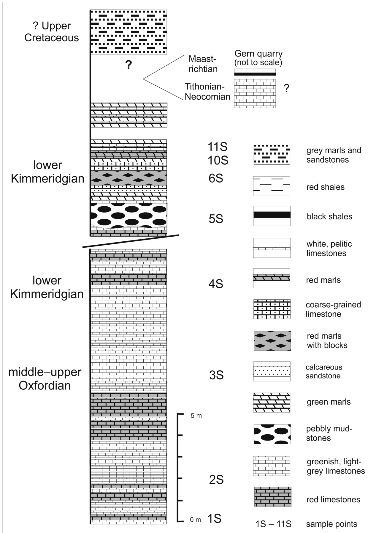
Figure 4: Interpretative column showing the lithology and the relationship between the exposed blocks within the Main Klippen Zone in the southern tributary of the Gernbach Stream in the Gern area.
