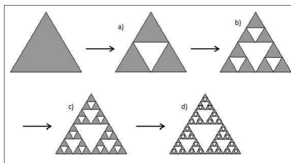
Figure 1: Fractal—the Sierpinski carpet (Falconer, 2003).
