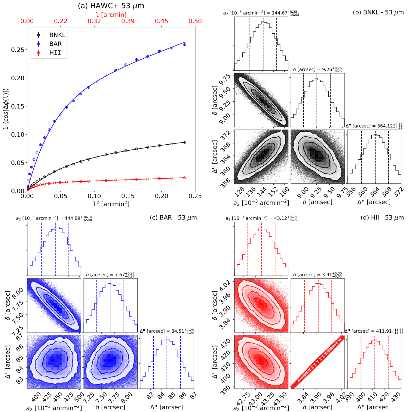
Figure 13. (a) DF for each OMC-1 region of interest using the 53 \mu\text{m} data. Data points (circles) and fits (solid lines) are color coded to match the region they represent: black, blue, red for BNKL, BAR, and H II region, respectively. Solid lines correspond to the best fit of data using Equation (12) and the parameters from Table 4. The model from Equation (12) only fits properly the DFs at spatial scales smaller than the ordered (large-scale) magnetic field, so the solid lines are shown only over the l -values used in each fit. (b)–(d) Results from the MCMC solver for each studied region.
