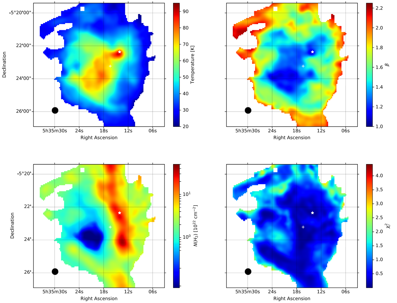
Figure 3. Clockwise from top left: the fitted temperatures, dust emissivity indices, \chi_r^2 values, and calculated column densities. All are smoothed to a 22'' resolution. The effective beam size is shown on the bottom left in each panel as a black filled circle. Only points with \chi_r^2 < 5 are shown. The white cross indicates the center of the Trapezium cluster, while the white star shows the location of the BN object.
